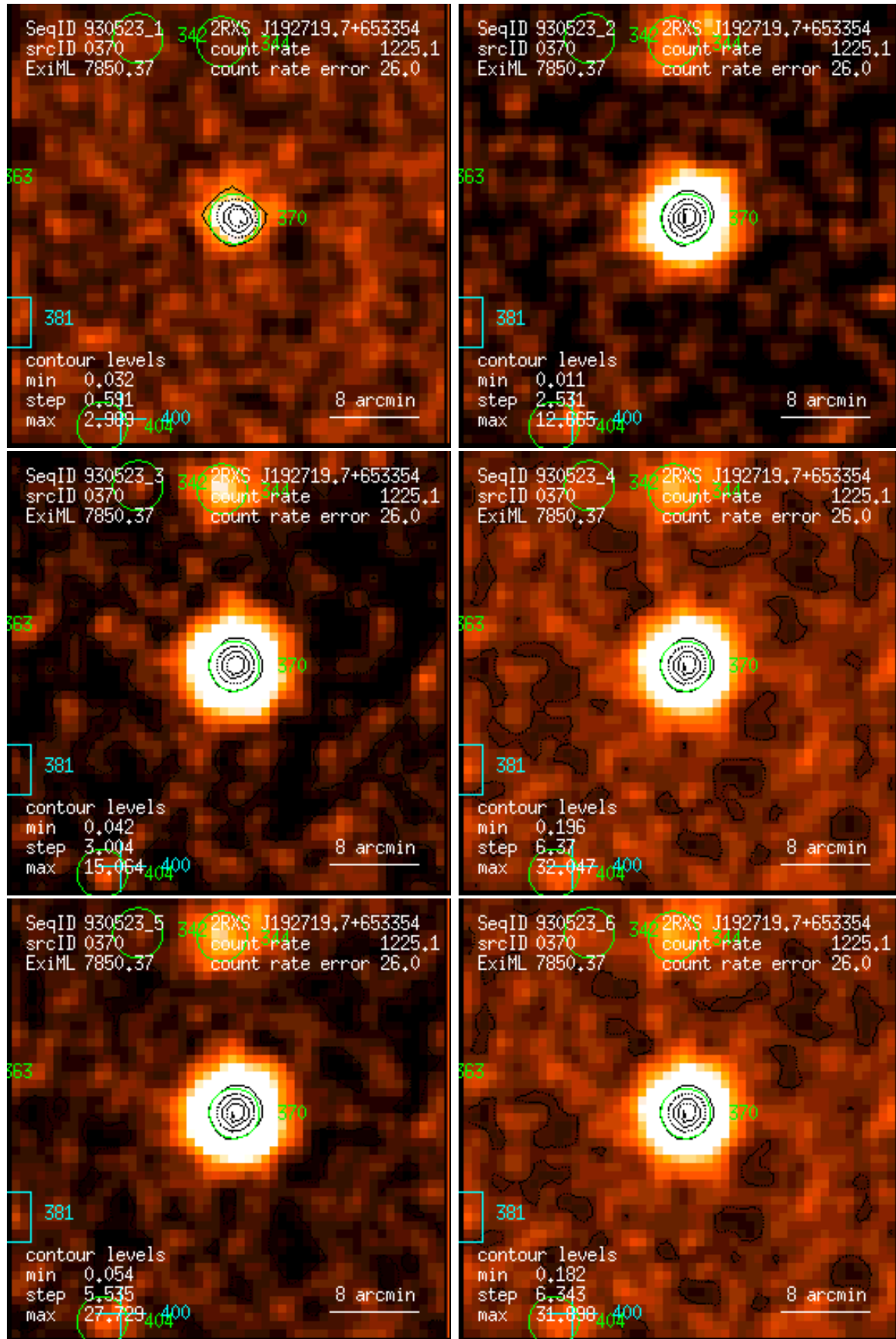
Figure 370: RASS 930523: detection 0370: band rate images, Gaussian filter: (1) PSPC channels 11 – 41, (2) 52 – 90, (3) 91 – 201, (4) 11 – 235, (5) 52 – 201, (6) 11 – 201. Broad band rates in counts/ks. Band rate contour levels in counts/ks/arcmin 2 .
