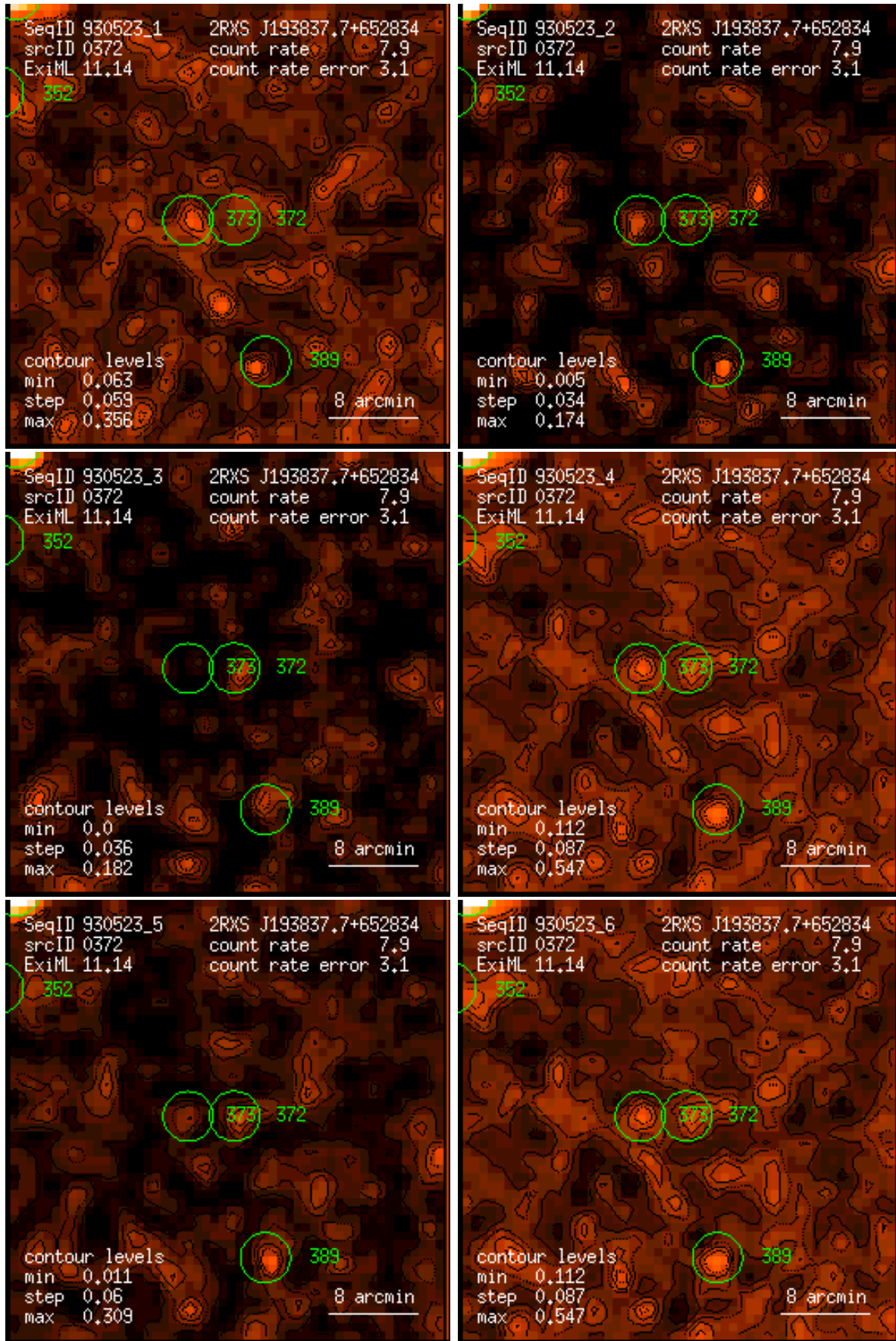
Figure 372: RASS 930523: detection 0372: band rate images, Gaussian filter: (1) PSPC channels 11 – 41, (2) 52 – 90, (3) 91 – 201, (4) 11 – 235, (5) 52 – 201, (6) 11 – 201. Broad band rates in counts/ks. Band rate contour levels in counts/ks/arcmin 2 .
