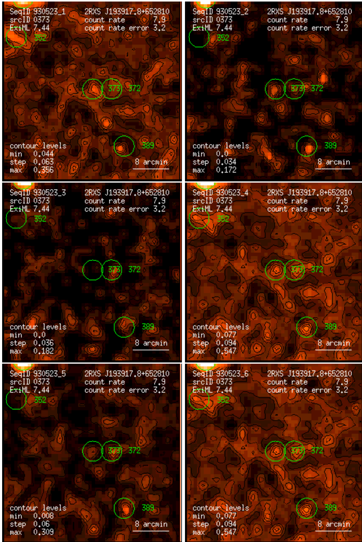
Figure 373: RASS 930523: detection 0373: band rate images, Gaussian filter: (1) PSPC channels 11 – 41, (2) 52 – 90, (3) 91 – 201, (4) 11 – 235, (5) 52 – 201, (6) 11 – 201. Broad band rates in counts/ks. Band rate contour levels in counts/ks/arcmin 2 .
