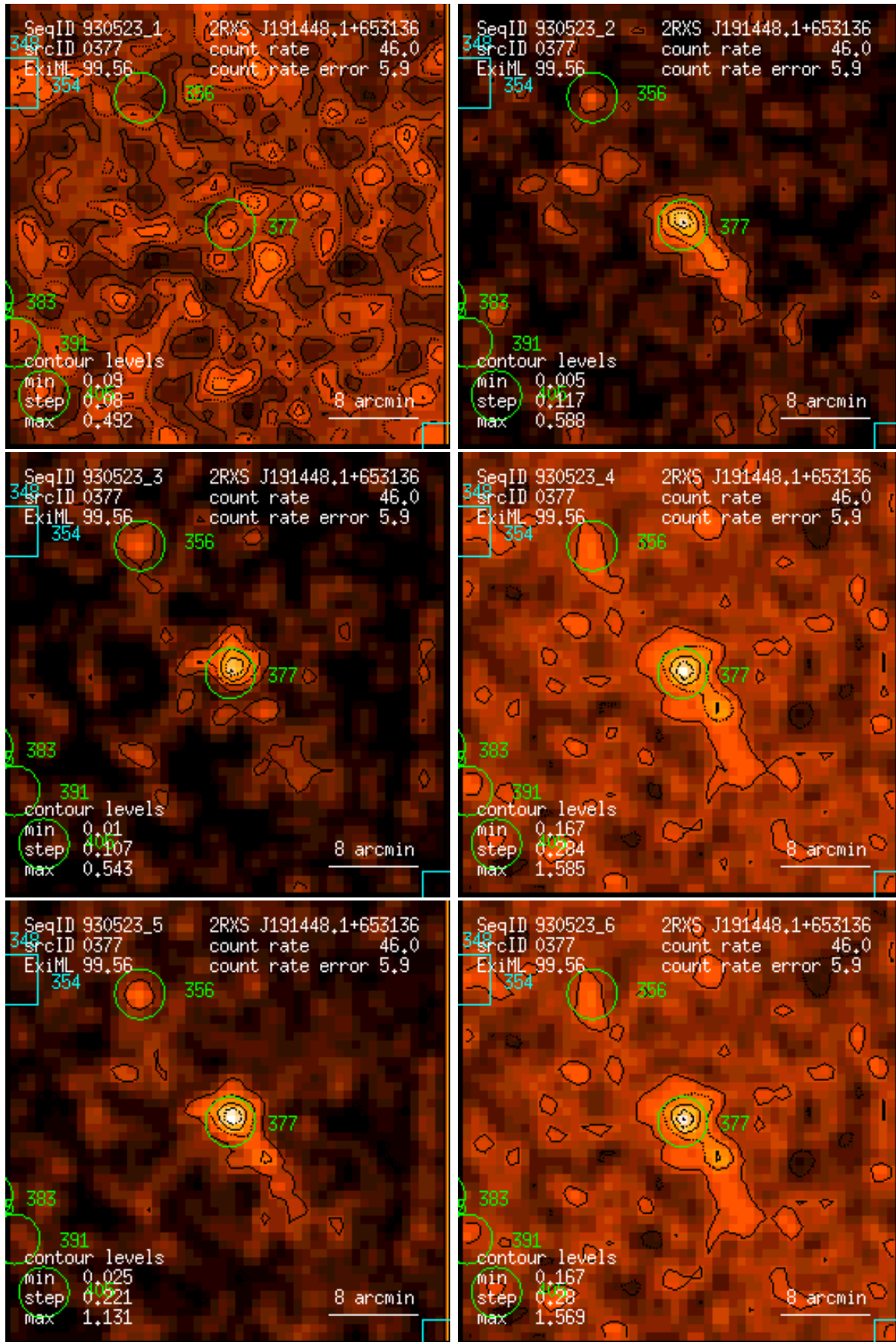
Figure 377: RASS 930523: detection 0377: band rate images, Gaussian filter: (1) PSPC channels 11 – 41, (2) 52 – 90, (3) 91 – 201, (4) 11 – 235, (5) 52 – 201, (6) 11 – 201. Broad band rates in counts/ks. Band rate contour levels in counts/ks/arcmin 2 .
