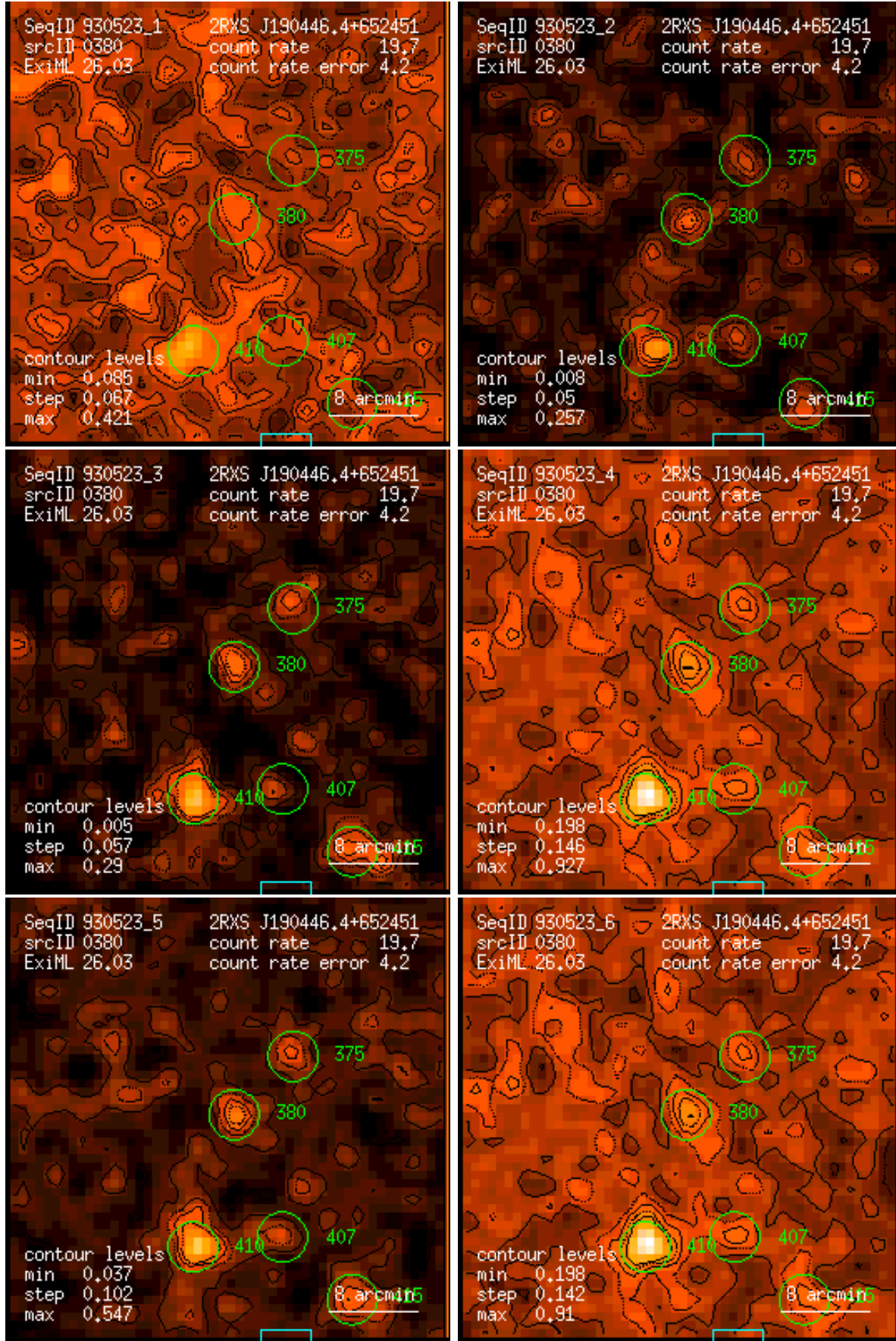
Figure 380: RASS 930523: detection 0380: band rate images, Gaussian filter: (1) PSPC channels 11 – 41, (2) 52 – 90, (3) 91 – 201, (4) 11 – 235, (5) 52 – 201, (6) 11 – 201. Broad band rates in counts/ks. Band rate contour levels in counts/ks/arcmin 2 .
