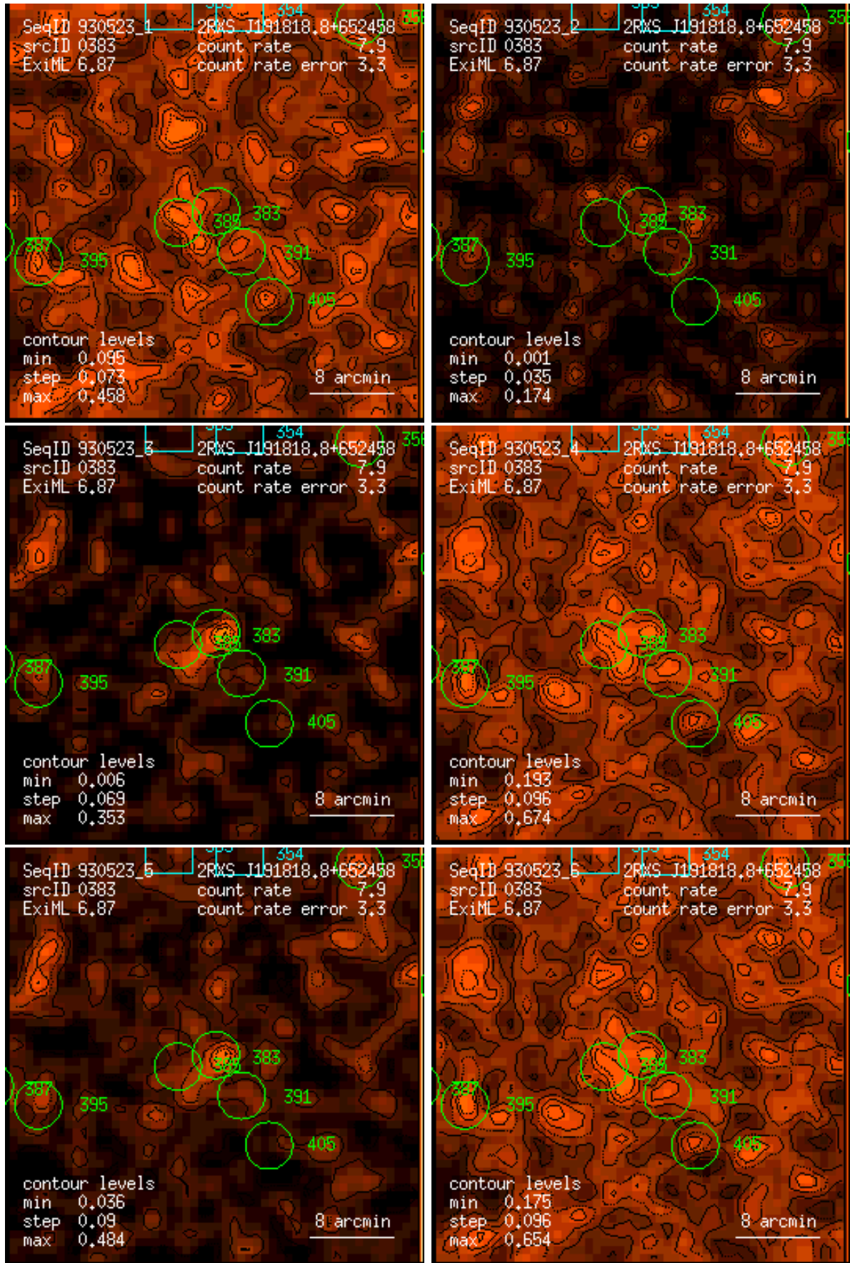
Figure 383: RASS 930523: detection 0383: band rate images, Gaussian filter: (1) PSPC channels 11 – 41, (2) 52 – 90, (3) 91 – 201, (4) 11 – 235, (5) 52 – 201, (6) 11 – 201. Broad band rates in counts/ks. Band rate contour levels in counts/ks/arcmin 2 .
