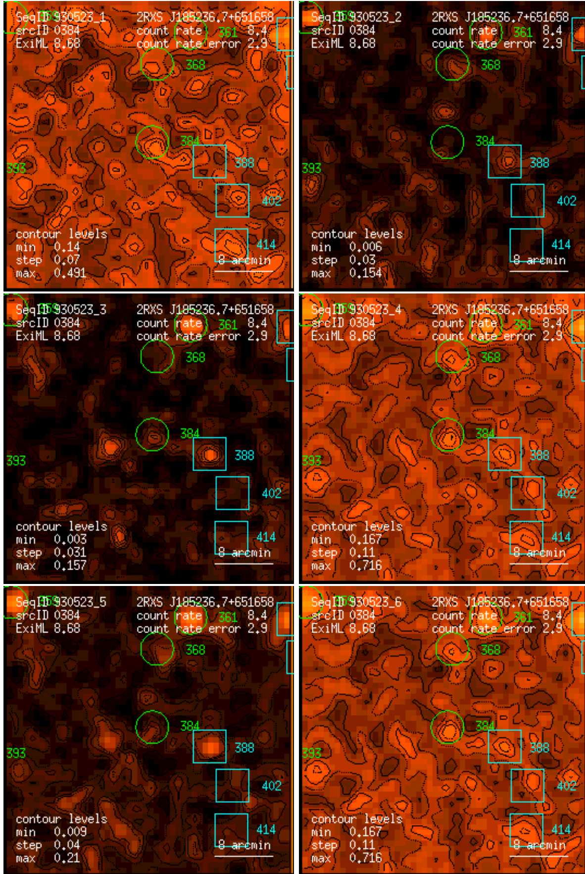
Figure 384: RASS 930523: detection 0384: band rate images, Gaussian filter: (1) PSPC channels 11 – 41, (2) 52 – 90, (3) 91 – 201, (4) 11 – 235, (5) 52 – 201, (6) 11 – 201. Broad band rates in counts/ks. Band rate contour levels in counts/ks/arcmin 2 .
