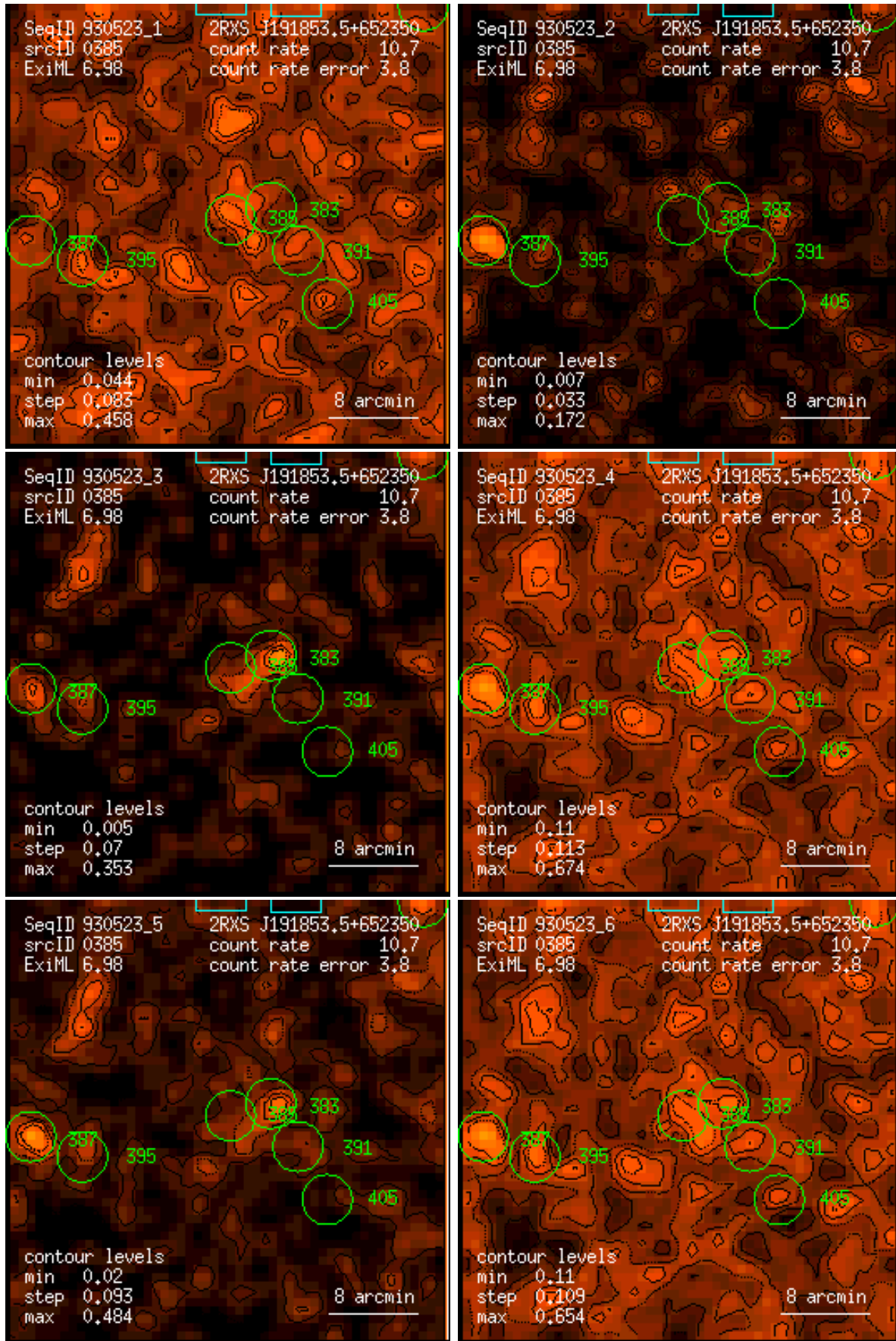
Figure 385: RASS 930523: detection 0385: band rate images, Gaussian filter: (1) PSPC channels 11 – 41, (2) 52 – 90, (3) 91 – 201, (4) 11 – 235, (5) 52 – 201, (6) 11 – 201. Broad band rates in counts/ks. Band rate contour levels in counts/ks/arcmin 2 .
