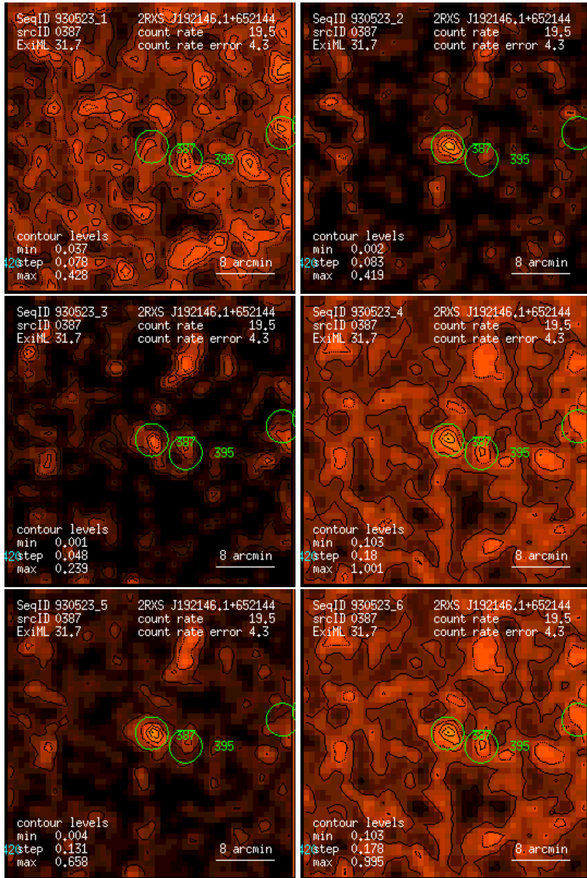
Figure 387: RASS 930523: detection 0387: band rate images, Gaussian filter: (1) PSPC channels 11 – 41, (2) 52 – 90, (3) 91 – 201, (4) 11 – 235, (5) 52 – 201, (6) 11 – 201. Broad band rates in counts/ks. Band rate contour levels in counts/ks/arcmin 2 .
