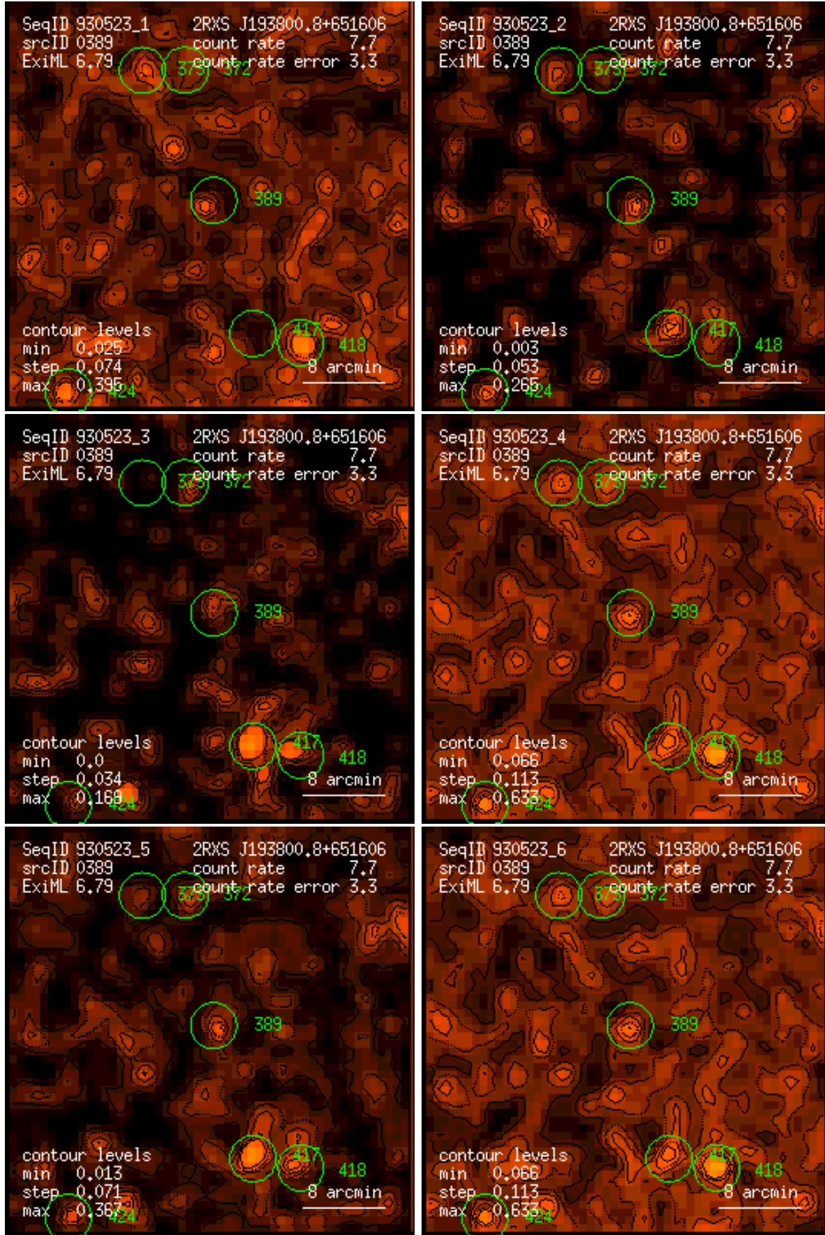
Figure 389: RASS 930523: detection 0389: band rate images, Gaussian filter: (1) PSPC channels 11 – 41, (2) 52 – 90, (3) 91 – 201, (4) 11 – 235, (5) 52 – 201, (6) 11 – 201. Broad band rates in counts/ks. Band rate contour levels in counts/ks/arcmin 2 .
