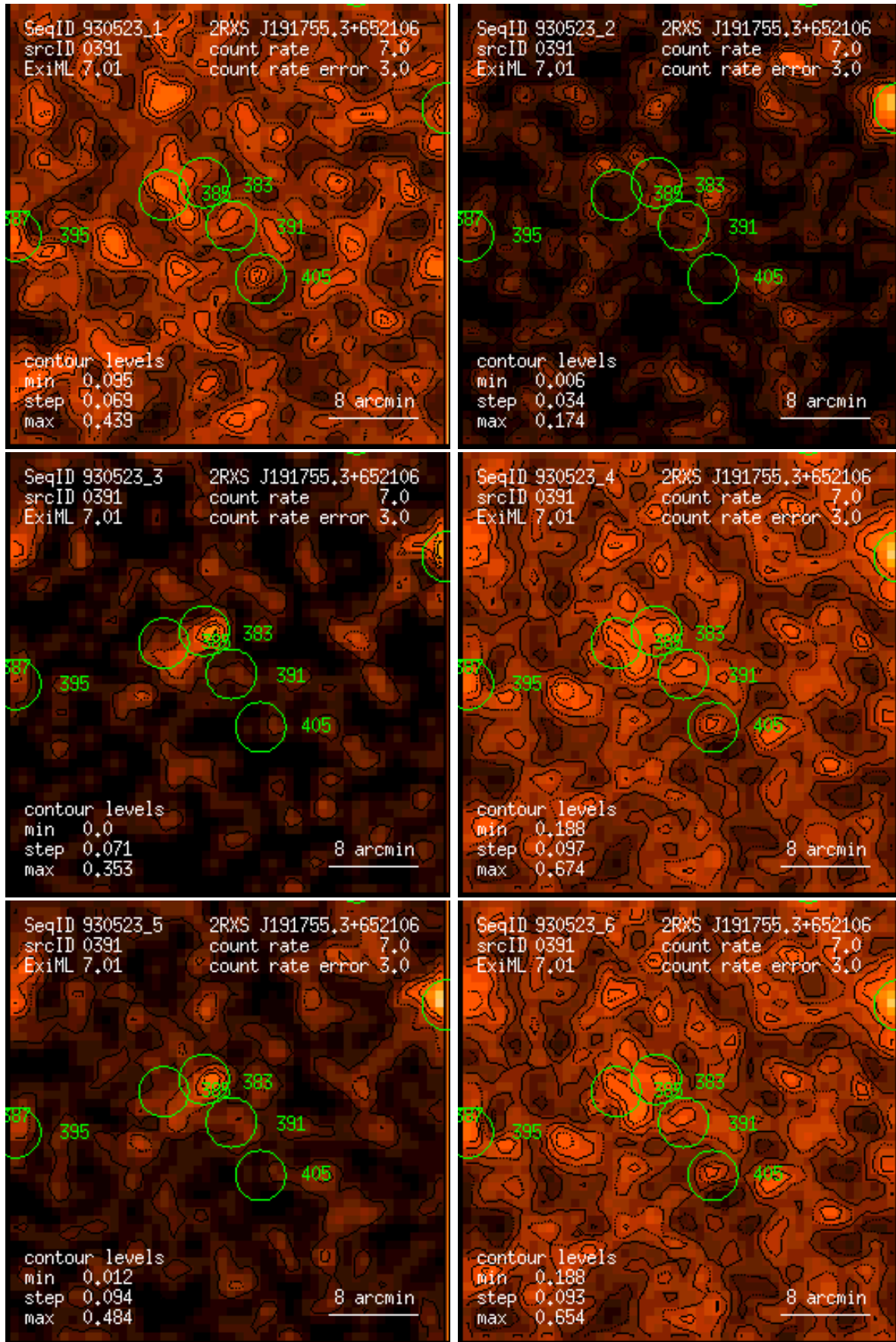
Figure 391: RASS 930523: detection 0391: band rate images, Gaussian filter: (1) PSPC channels 11 – 41, (2) 52 – 90, (3) 91 – 201, (4) 11 – 235, (5) 52 – 201, (6) 11 – 201. Broad band rates in counts/ks. Band rate contour levels in counts/ks/arcmin 2 .
