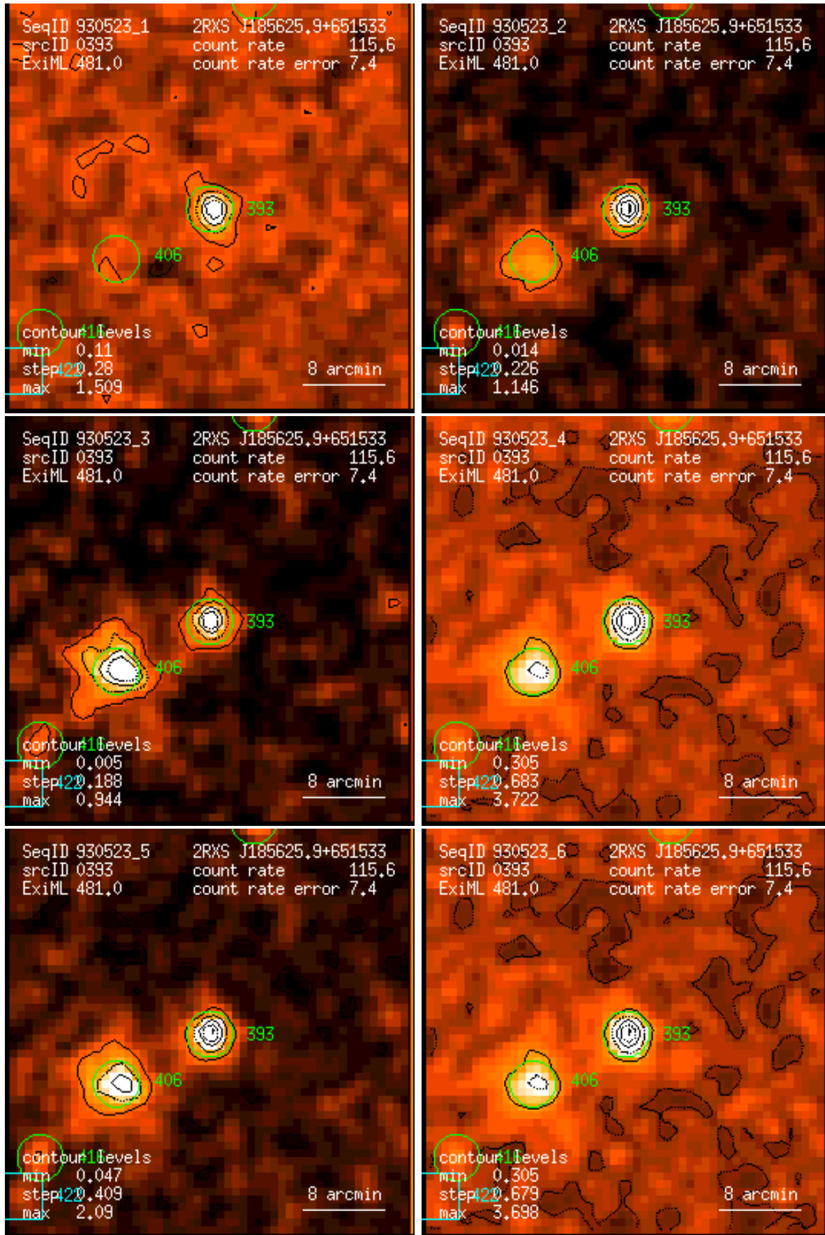
Figure 393: RASS 930523: detection 0393: band rate images, Gaussian filter: (1) PSPC channels 11 – 41, (2) 52 – 90, (3) 91 – 201, (4) 11 – 235, (5) 52 – 201, (6) 11 – 201. Broad band rates in counts/ks. Band rate contour levels in counts/ks/arcmin 2 .
