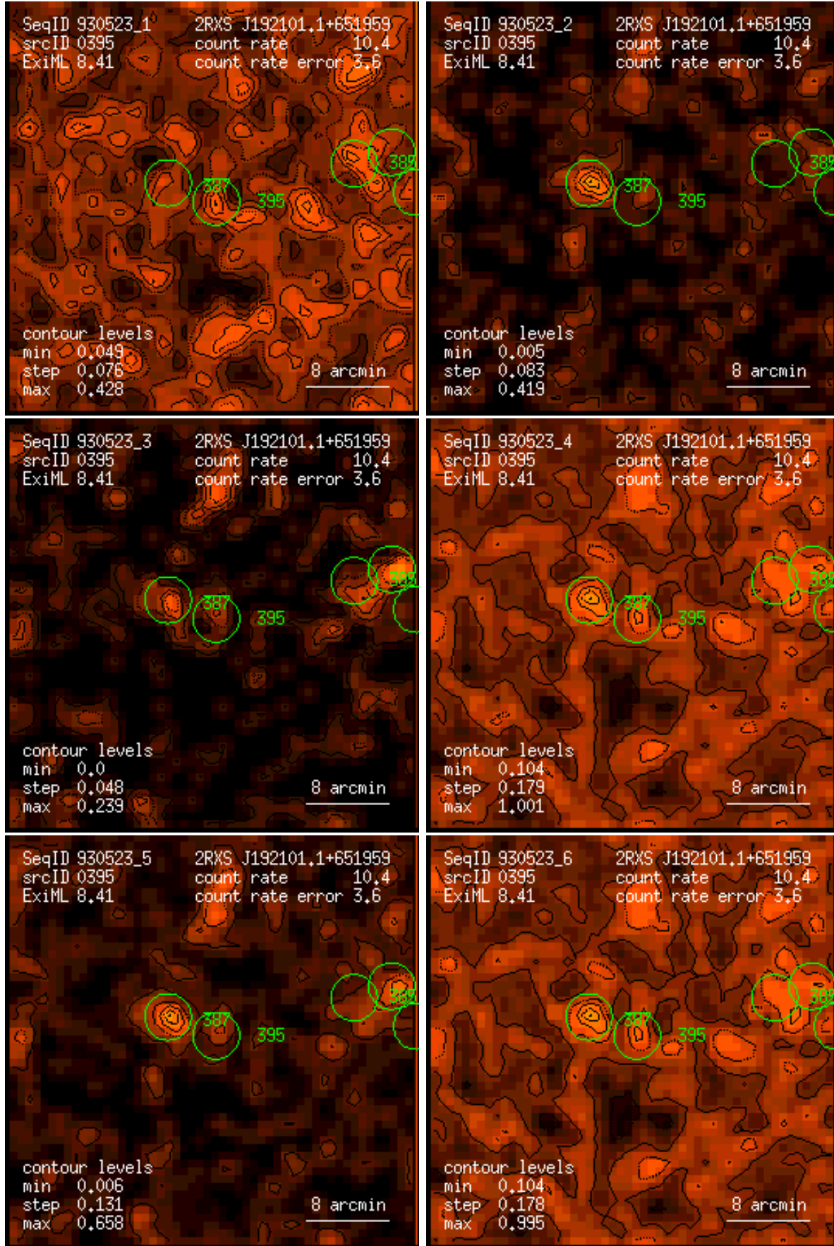
Figure 395: RASS 930523: detection 0395: band rate images, Gaussian filter: (1) PSPC channels 11 – 41, (2) 52 – 90, (3) 91 – 201, (4) 11 – 235, (5) 52 – 201, (6) 11 – 201. Broad band rates in counts/ks. Band rate contour levels in counts/ks/arcmin 2 .
