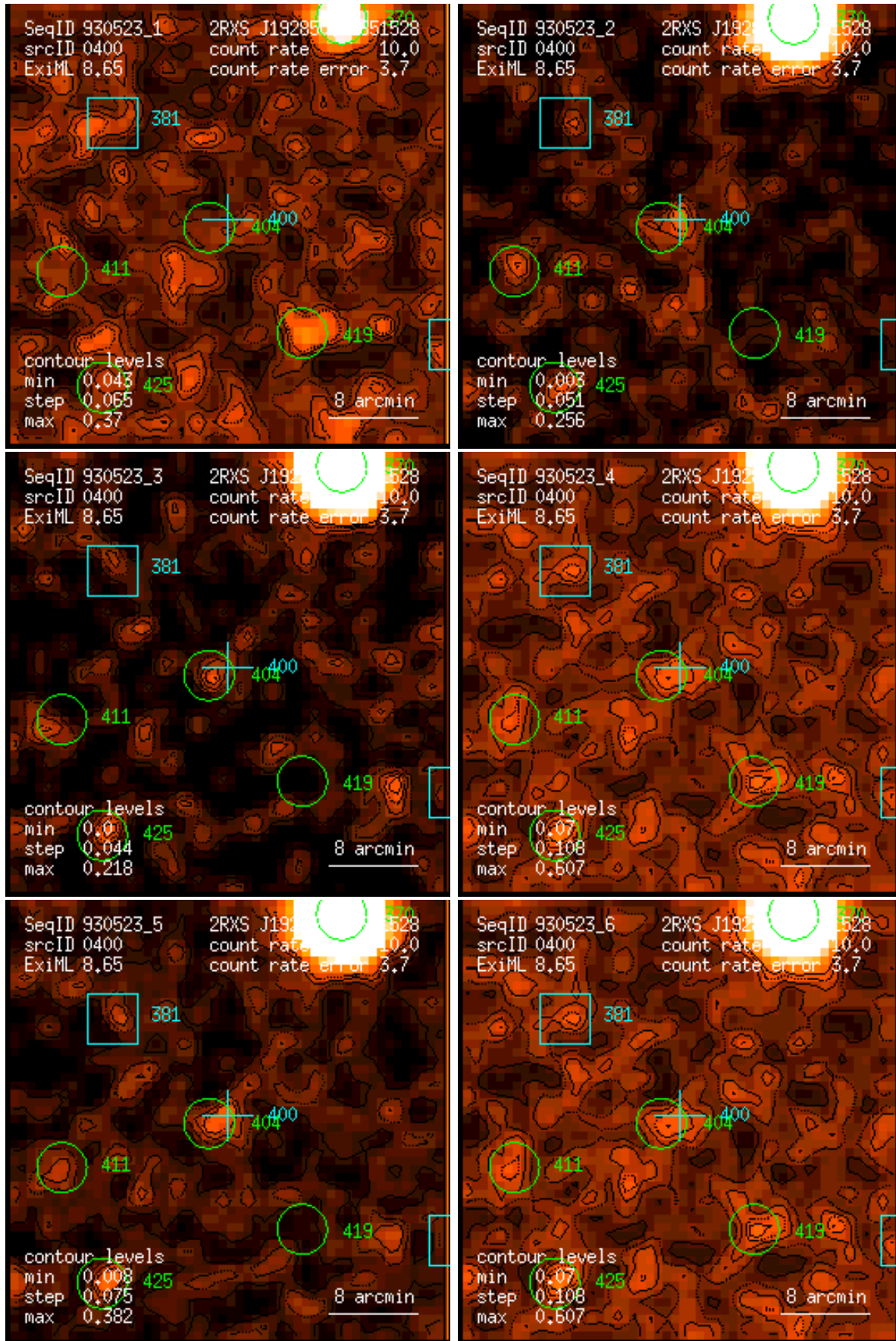
Figure 400: RASS 930523: detection 0400: band rate images, Gaussian filter: (1) PSPC channels 11 – 41, (2) 52 – 90, (3) 91 – 201, (4) 11 – 235, (5) 52 – 201, (6) 11 – 201. Broad band rates in counts/ks. Band rate contour levels in counts/ks/arcmin 2 .
