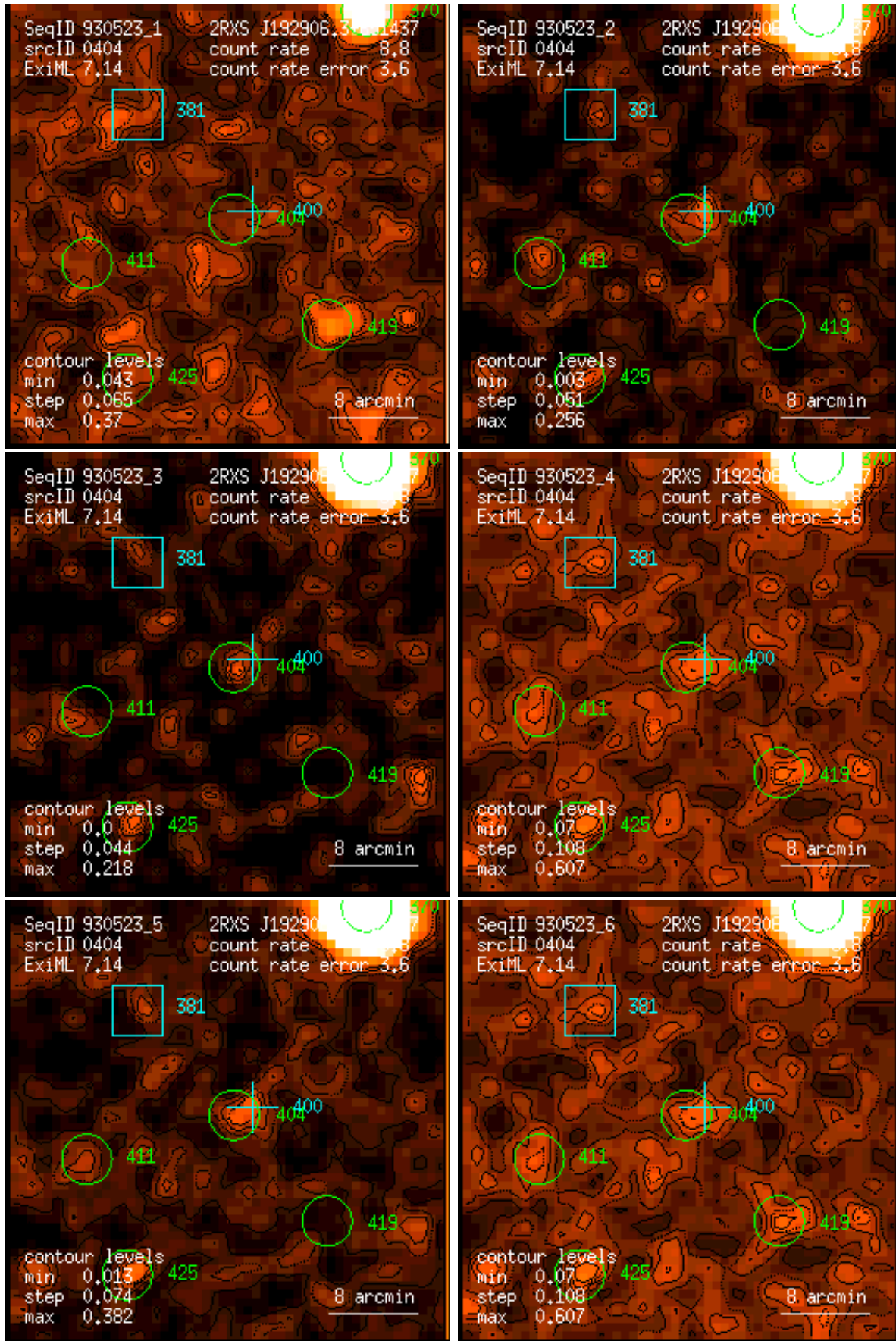
Figure 404: RASS 930523: detection 0404: band rate images, Gaussian filter: (1) PSPC channels 11 – 41, (2) 52 – 90, (3) 91 – 201, (4) 11 – 235, (5) 52 – 201, (6) 11 – 201. Broad band rates in counts/ks. Band rate contour levels in counts/ks/arcmin 2 .
