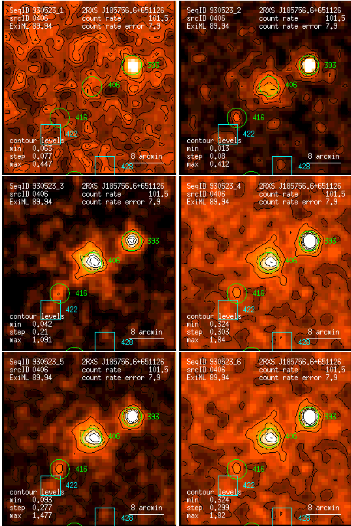
Figure 406: RASS 930523: detection 0406: band rate images, Gaussian filter: (1) PSPC channels 11 – 41, (2) 52 – 90, (3) 91 – 201, (4) 11 – 235, (5) 52 – 201, (6) 11 – 201. Broad band rates in counts/ks. Band rate contour levels in counts/ks/arcmin 2 .
