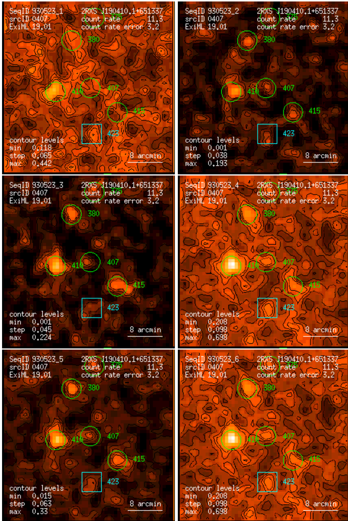
Figure 407: RASS 930523: detection 0407: band rate images, Gaussian filter: (1) PSPC channels 11 – 41, (2) 52 – 90, (3) 91 – 201, (4) 11 – 235, (5) 52 – 201, (6) 11 – 201. Broad band rates in counts/ks. Band rate contour levels in counts/ks/arcmin 2 .
