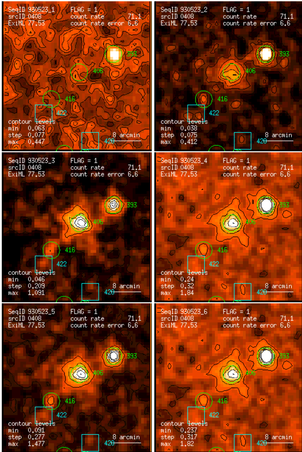
Figure 408: RASS 930523: detection 0408: band rate images, Gaussian filter: (1) PSPC channels 11 – 41, (2) 52 – 90, (3) 91 – 201, (4) 11 – 235, (5) 52 – 201, (6) 11 – 201. Broad band rates in counts/ks. Band rate contour levels in counts/ks/arcmin 2 .
