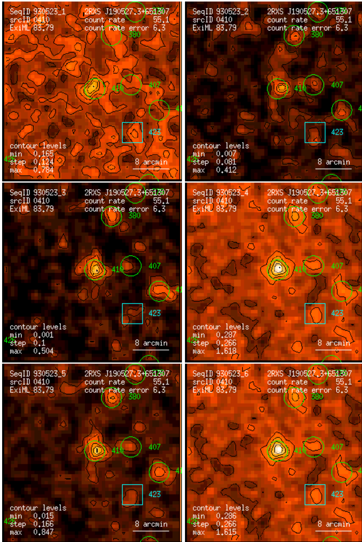
Figure 410: RASS 930523: detection 0410: band rate images, Gaussian filter: (1) PSPC channels 11 – 41, (2) 52 – 90, (3) 91 – 201, (4) 11 – 235, (5) 52 – 201, (6) 11 – 201. Broad band rates in counts/ks. Band rate contour levels in counts/ks/arcmin 2 .
