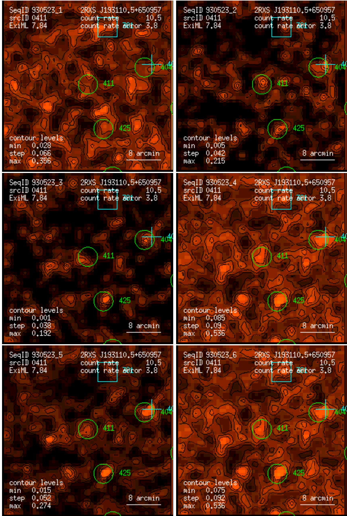
Figure 411: RASS 930523: detection 0411: band rate images, Gaussian filter: (1) PSPC channels 11 – 41, (2) 52 – 90, (3) 91 – 201, (4) 11 – 235, (5) 52 – 201, (6) 11 – 201. Broad band rates in counts/ks. Band rate contour levels in counts/ks/arcmin 2 .
