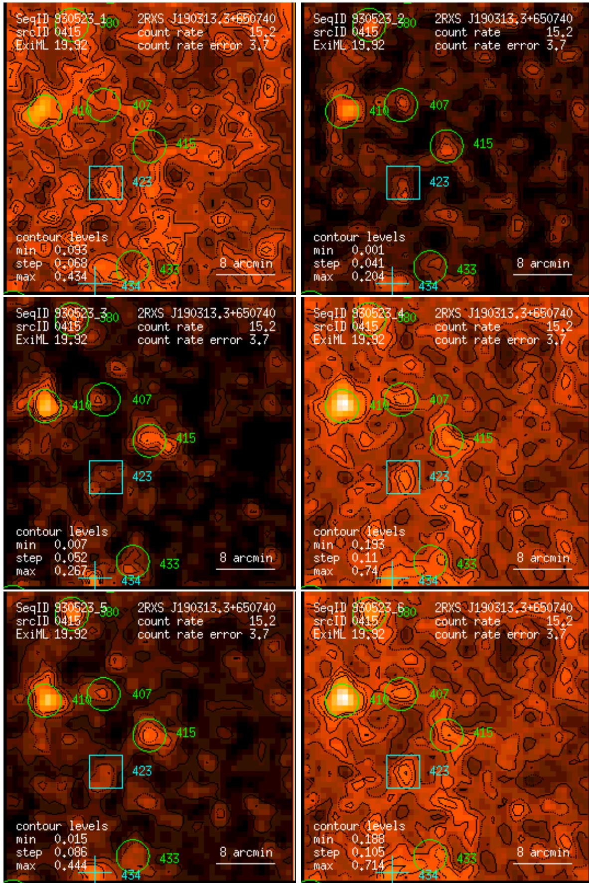
Figure 415: RASS 930523: detection 0415: band rate images, Gaussian filter: (1) PSPC channels 11 – 41, (2) 52 – 90, (3) 91 – 201, (4) 11 – 235, (5) 52 – 201, (6) 11 – 201. Broad band rates in counts/ks. Band rate contour levels in counts/ks/arcmin 2 .
