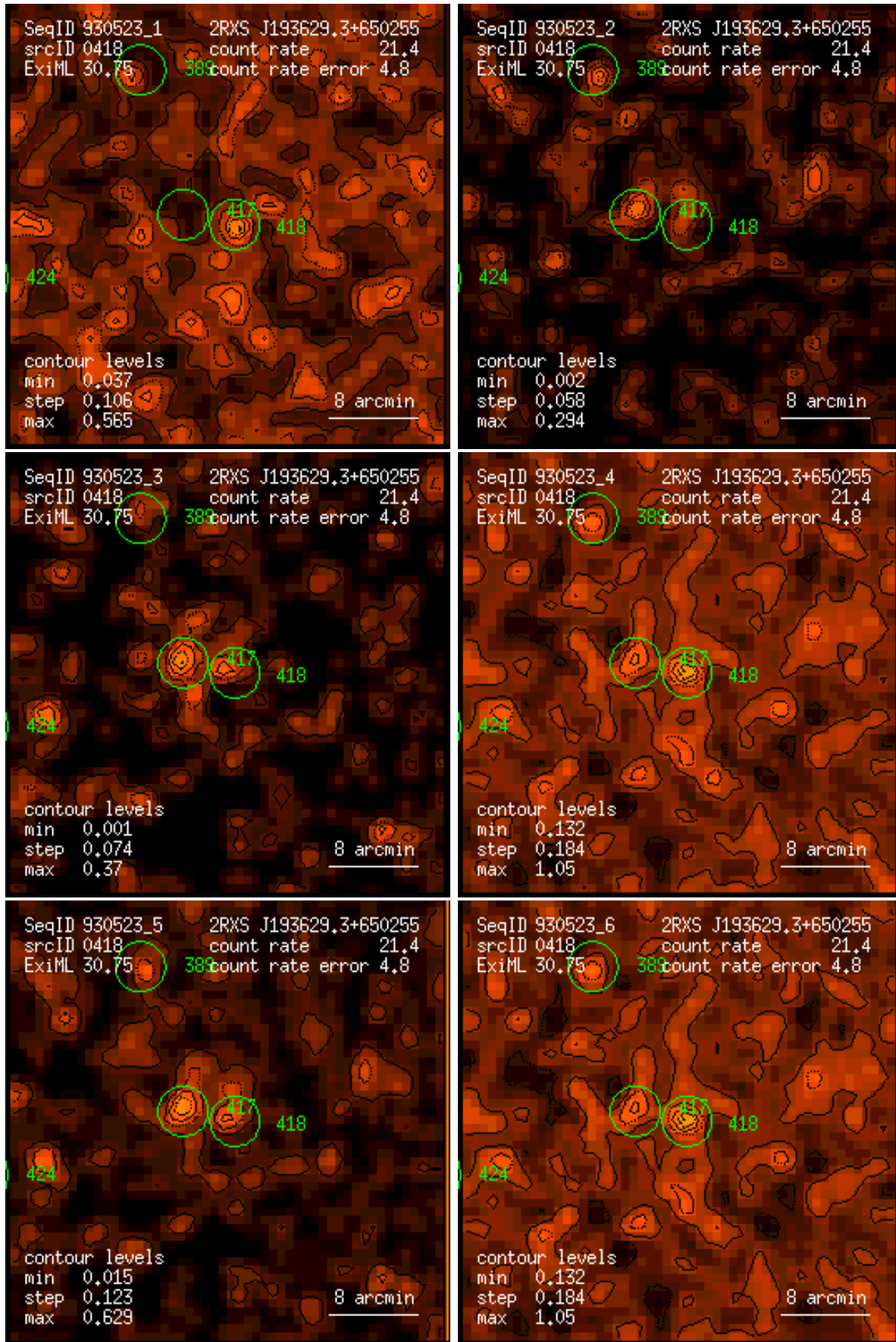
Figure 418: RASS 930523: detection 0418: band rate images, Gaussian filter: (1) PSPC channels 11 – 41, (2) 52 – 90, (3) 91 – 201, (4) 11 – 235, (5) 52 – 201, (6) 11 – 201. Broad band rates in counts/ks. Band rate contour levels in counts/ks/arcmin 2 .
