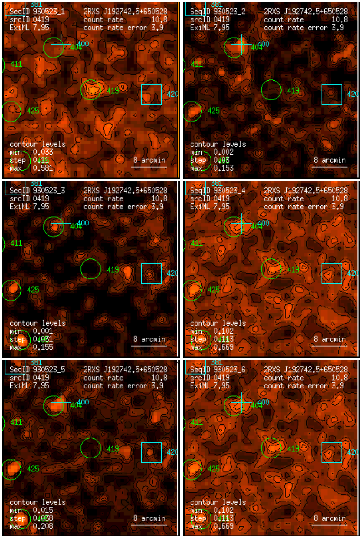
Figure 419: RASS 930523: detection 0419: band rate images, Gaussian filter: (1) PSPC channels 11 – 41, (2) 52 – 90, (3) 91 – 201, (4) 11 – 235, (5) 52 – 201, (6) 11 – 201. Broad band rates in counts/ks. Band rate contour levels in counts/ks/arcmin 2 .
