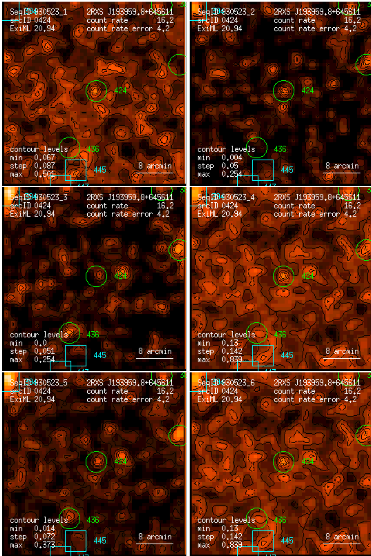
Figure 424: RASS 930523: detection 0424: band rate images, Gaussian filter: (1) PSPC channels 11 – 41, (2) 52 – 90, (3) 91 – 201, (4) 11 – 235, (5) 52 – 201, (6) 11 – 201. Broad band rates in counts/ks. Band rate contour levels in counts/ks/arcmin 2 .
