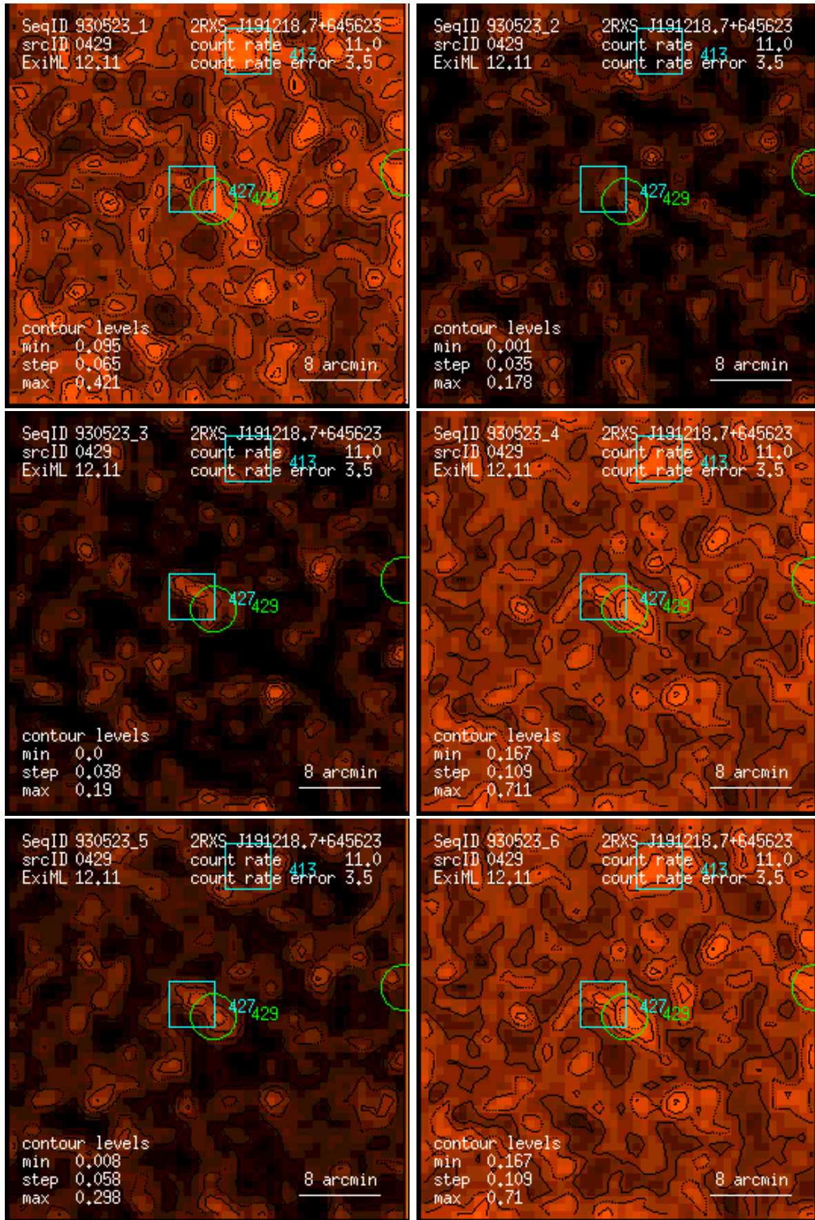
Figure 429: RASS 930523: detection 0429: band rate images, Gaussian filter: (1) PSPC channels 11 – 41, (2) 52 – 90, (3) 91 – 201, (4) 11 – 235, (5) 52 – 201, (6) 11 – 201. Broad band rates in counts/ks. Band rate contour levels in counts/ks/arcmin 2 .
