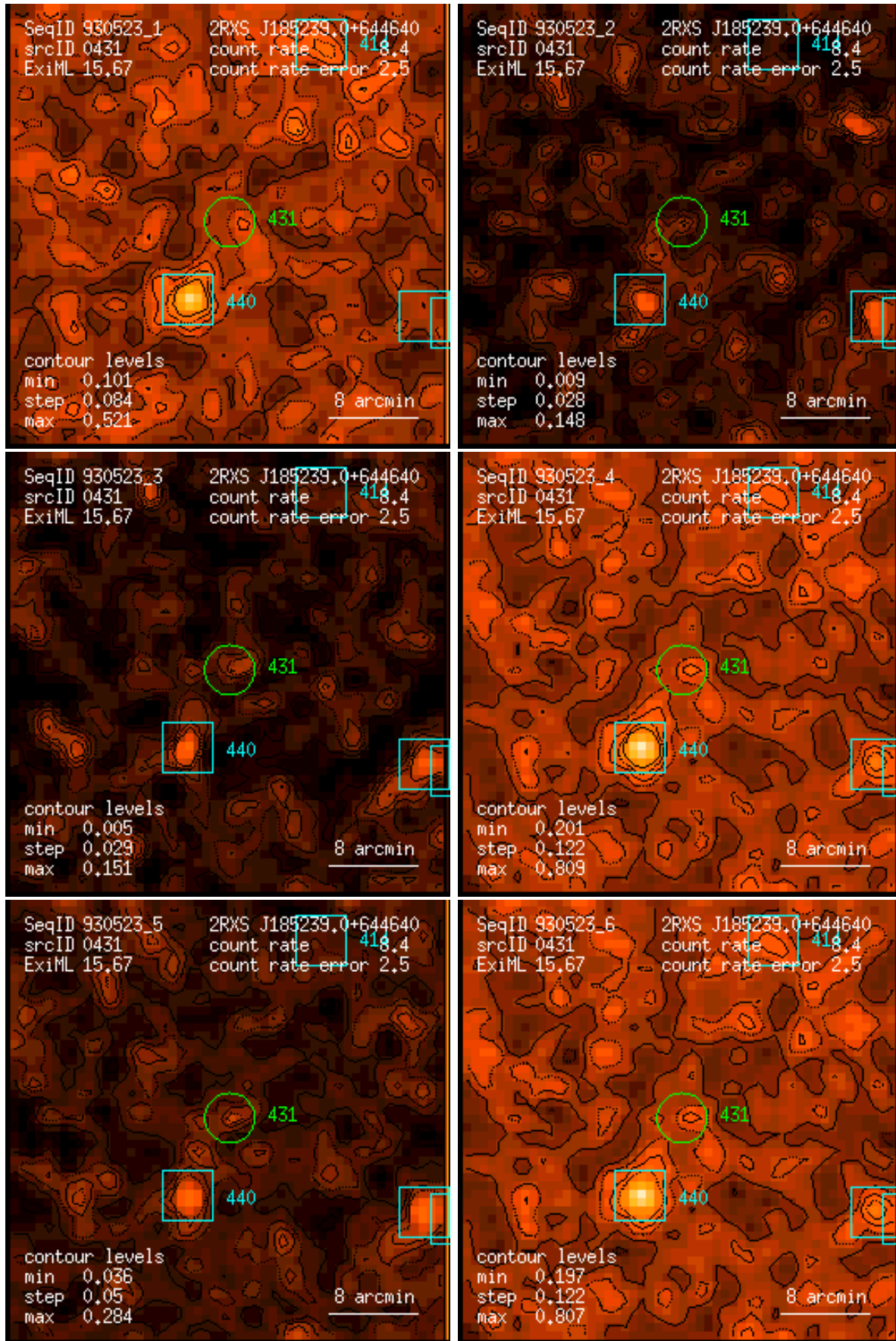
Figure 431: RASS 930523: detection 0431: band rate images, Gaussian filter: (1) PSPC channels 11 – 41, (2) 52 – 90, (3) 91 – 201, (4) 11 – 235, (5) 52 – 201, (6) 11 – 201. Broad band rates in counts/ks. Band rate contour levels in counts/ks/arcmin 2 .
