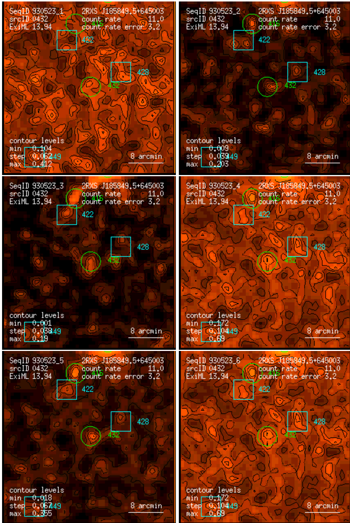
Figure 432: RASS 930523: detection 0432: band rate images, Gaussian filter: (1) PSPC channels 11 – 41, (2) 52 – 90, (3) 91 – 201, (4) 11 – 235, (5) 52 – 201, (6) 11 – 201. Broad band rates in counts/ks. Band rate contour levels in counts/ks/arcmin 2 .
