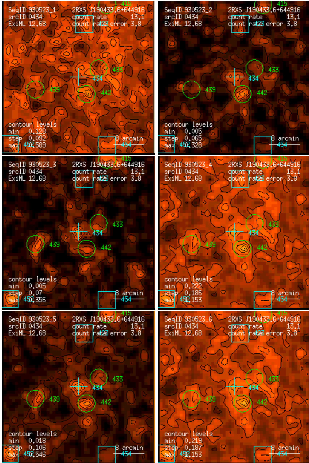
Figure 434: RASS 930523: detection 0434: band rate images, Gaussian filter: (1) PSPC channels 11 – 41, (2) 52 – 90, (3) 91 – 201, (4) 11 – 235, (5) 52 – 201, (6) 11 – 201. Broad band rates in counts/ks. Band rate contour levels in counts/ks/arcmin 2 .
