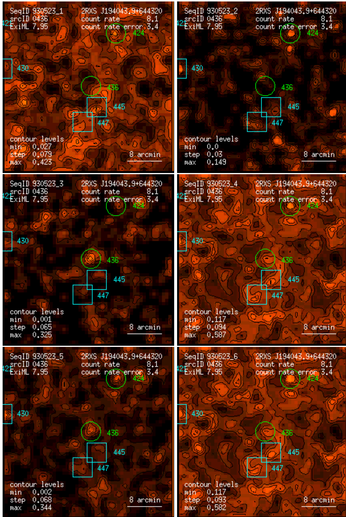
Figure 436: RASS 930523: detection 0436: band rate images, Gaussian filter: (1) PSPC channels 11 – 41, (2) 52 – 90, (3) 91 – 201, (4) 11 – 235, (5) 52 – 201, (6) 11 – 201. Broad band rates in counts/ks. Band rate contour levels in counts/ks/arcmin 2 .
