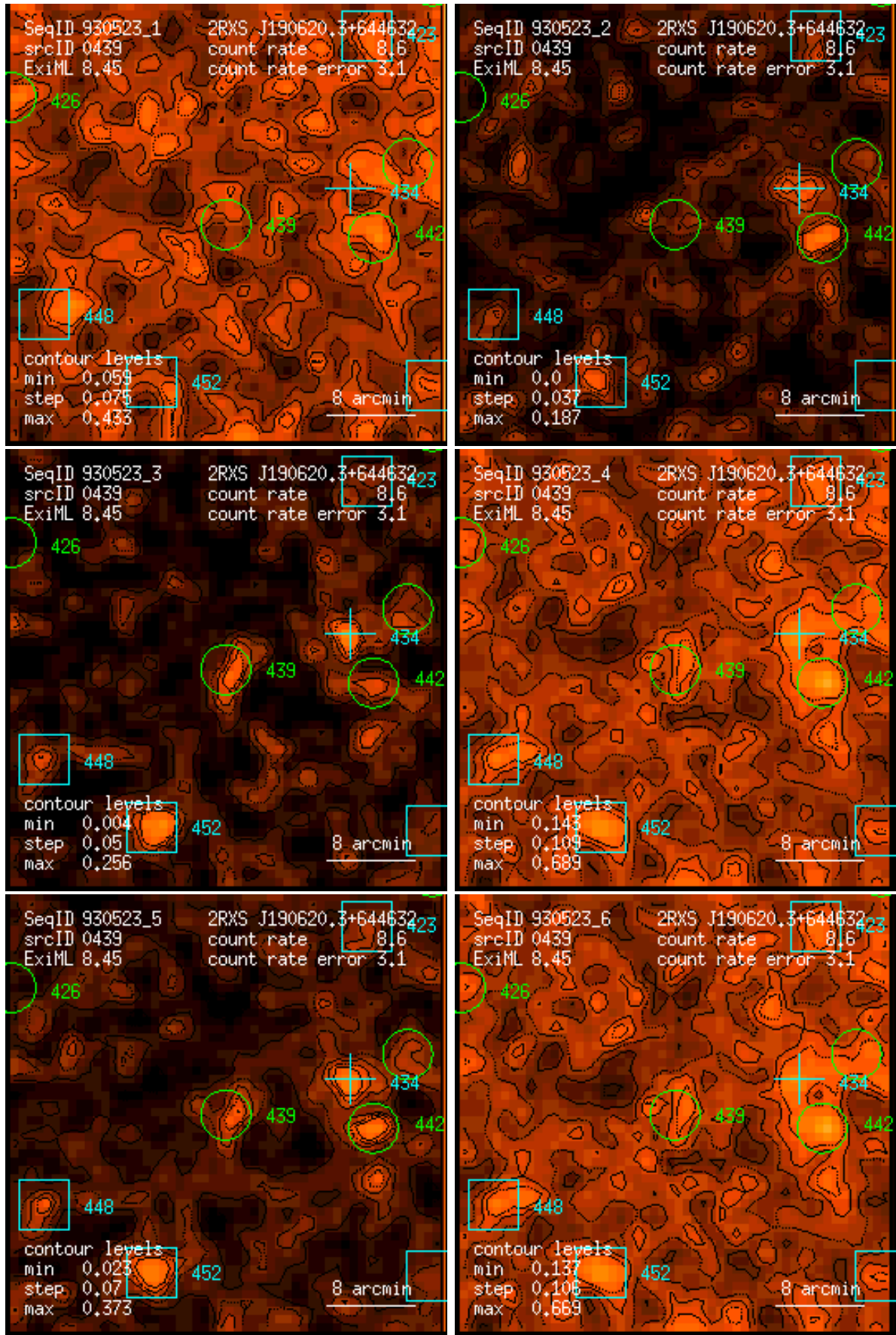
Figure 439: RASS 930523: detection 0439: band rate images, Gaussian filter: (1) PSPC channels 11 – 41, (2) 52 – 90, (3) 91 – 201, (4) 11 – 235, (5) 52 – 201, (6) 11 – 201. Broad band rates in counts/ks. Band rate contour levels in counts/ks/arcmin 2 .
