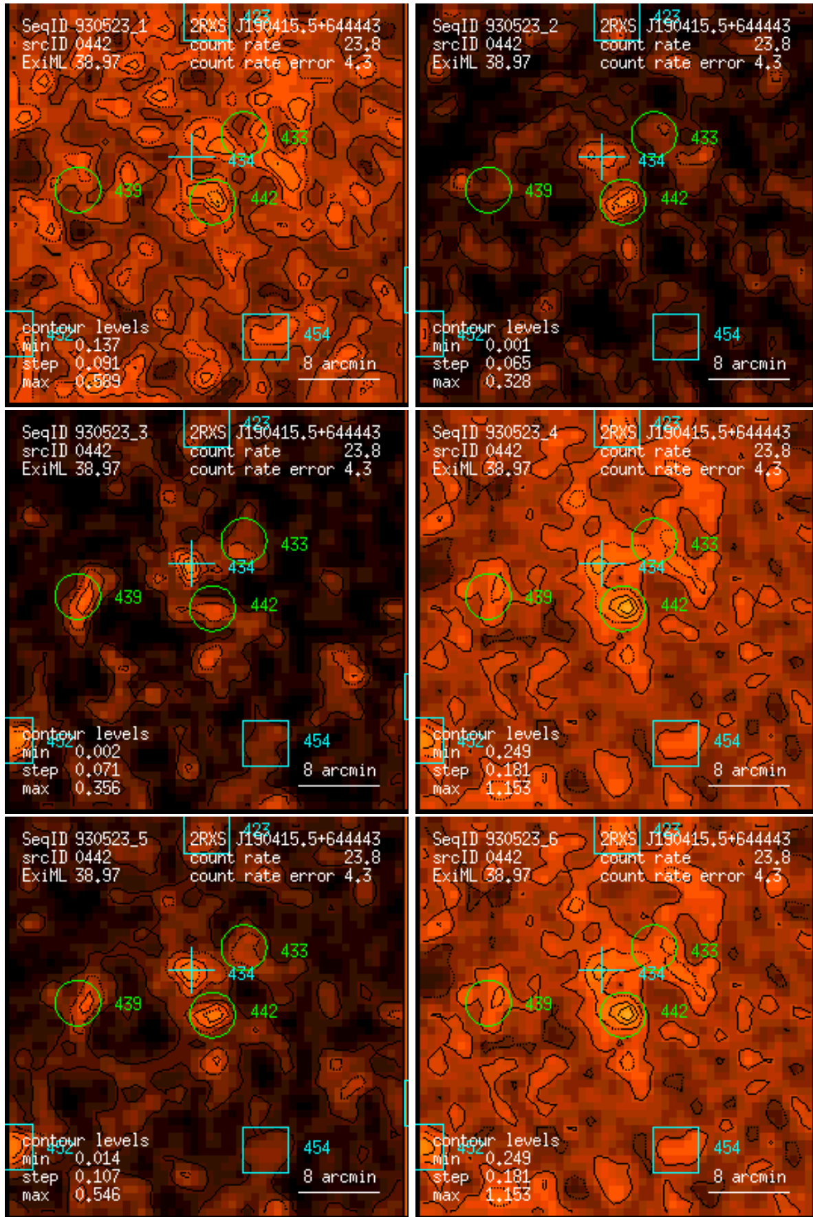
Figure 442: RASS 930523: detection 0442: band rate images, Gaussian filter: (1) PSPC channels 11 – 41, (2) 52 – 90, (3) 91 – 201, (4) 11 – 235, (5) 52 – 201, (6) 11 – 201. Broad band rates in counts/ks. Band rate contour levels in counts/ks/arcmin 2 .
