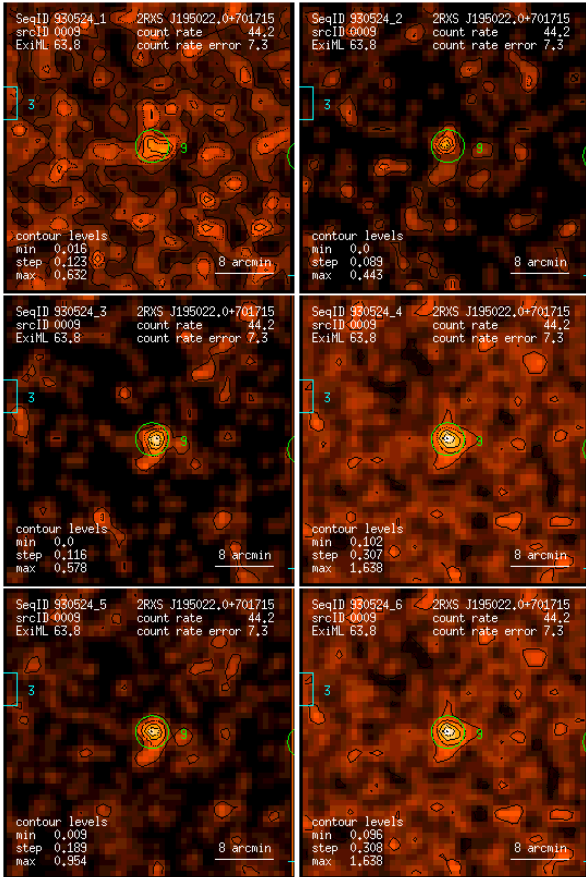
Figure 9: RASS 930524: detection 0009: band rate images, Gaussian filter: (1) PSPC channels 11 – 41, (2) 52 – 90, (3) 91 – 201, (4) 11 – 235, (5) 52 – 201, (6) 11 – 201. Broad band rates in counts/ks. Band rate contour levels in counts/ks/arcmin 2 .
