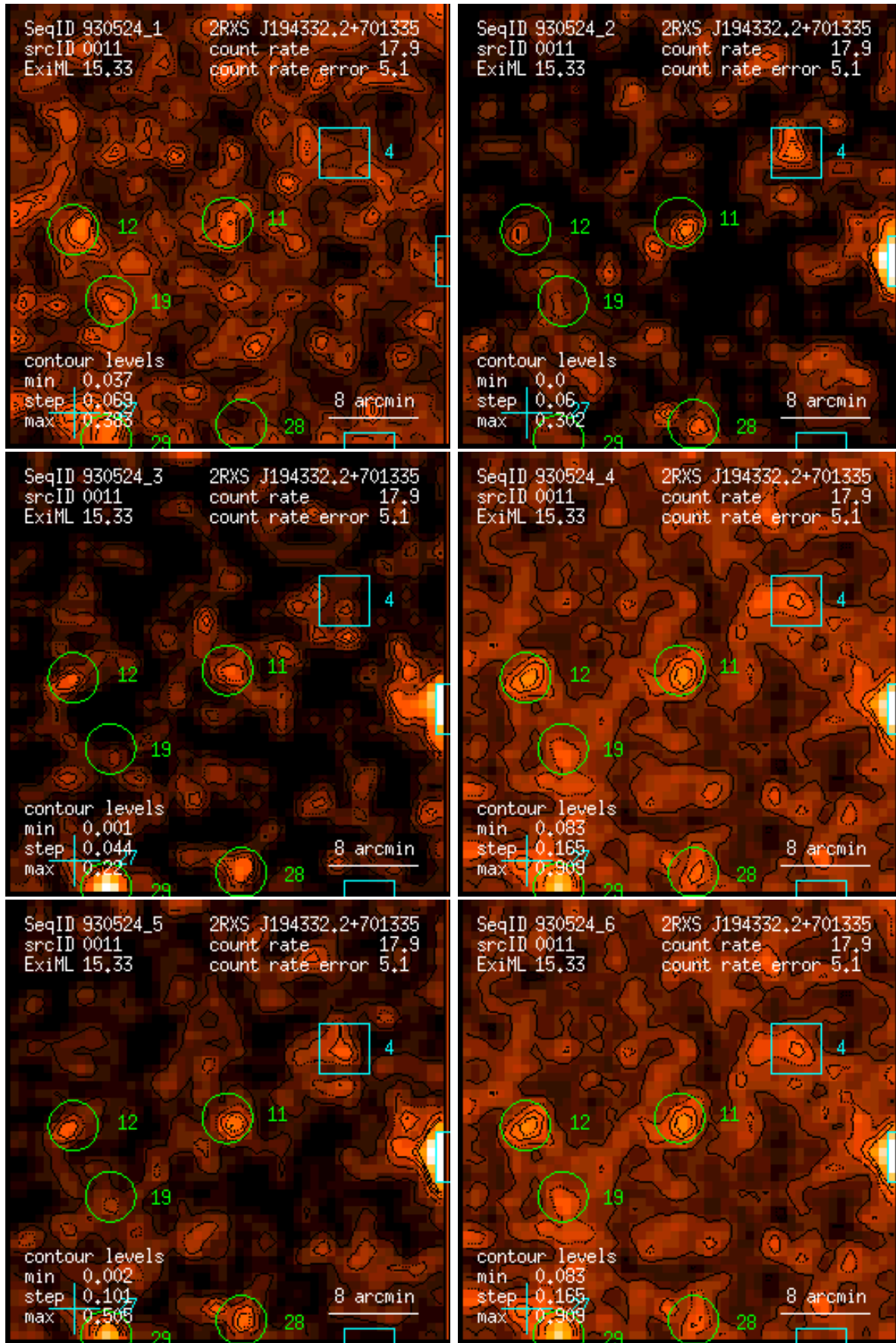
Figure 11: RASS 930524: detection 0011: band rate images, Gaussian filter: (1) PSPC channels 11 – 41, (2) 52 – 90, (3) 91 – 201, (4) 11 – 235, (5) 52 – 201, (6) 11 – 201. Broad band rates in counts/ks. Band rate contour levels in counts/ks/arcmin 2 .
