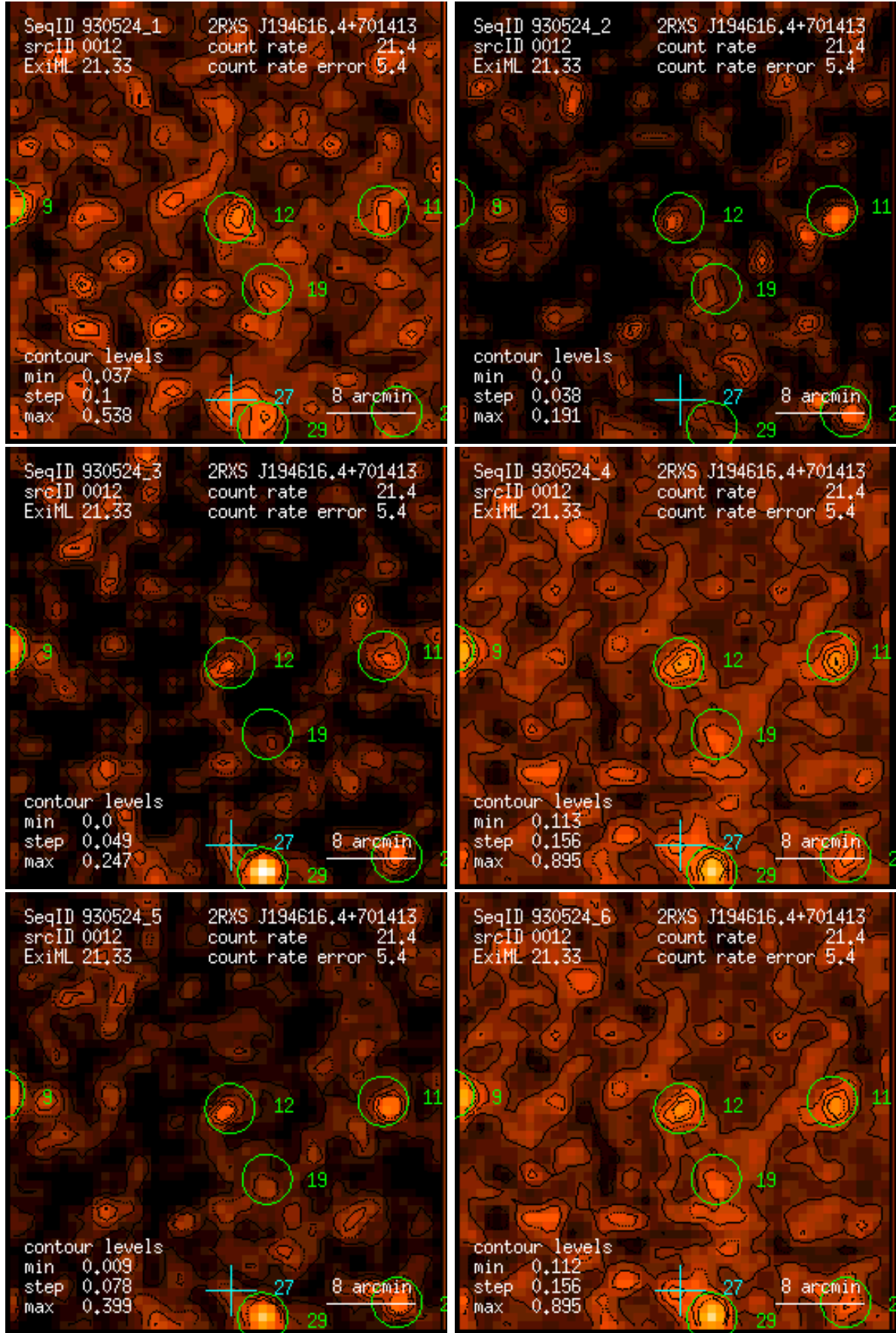
Figure 12: RASS 930524: detection 0012: band rate images, Gaussian filter: (1) PSPC channels 11 – 41, (2) 52 – 90, (3) 91 – 201, (4) 11 – 235, (5) 52 – 201, (6) 11 – 201. Broad band rates in counts/ks. Band rate contour levels in counts/ks/arcmin 2 .
