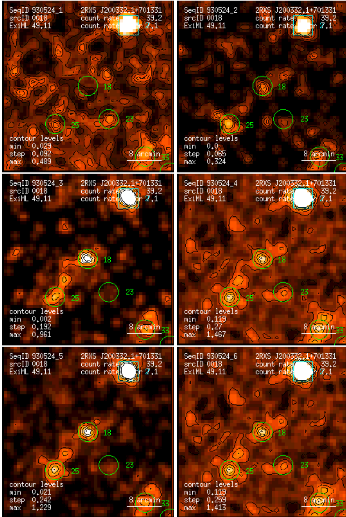
Figure 18: RASS 930524: detection 0018: band rate images, Gaussian filter: (1) PSPC channels 11 – 41, (2) 52 – 90, (3) 91 – 201, (4) 11 – 235, (5) 52 – 201, (6) 11 – 201. Broad band rates in counts/ks. Band rate contour levels in counts/ks/arcmin 2 .
