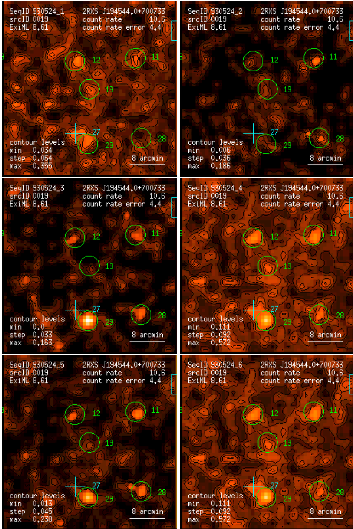
Figure 19: RASS 930524: detection 0019: band rate images, Gaussian filter: (1) PSPC channels 11 – 41, (2) 52 – 90, (3) 91 – 201, (4) 11 – 235, (5) 52 – 201, (6) 11 – 201. Broad band rates in counts/ks. Band rate contour levels in counts/ks/arcmin 2 .
