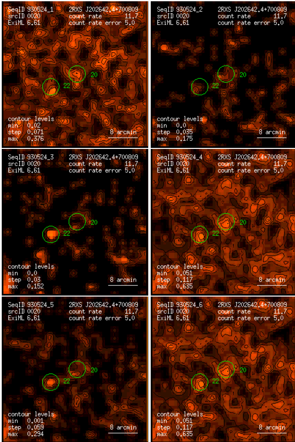
Figure 20: RASS 930524: detection 0020: band rate images, Gaussian filter: (1) PSPC channels 11 – 41, (2) 52 – 90, (3) 91 – 201, (4) 11 – 235, (5) 52 – 201, (6) 11 – 201. Broad band rates in counts/ks. Band rate contour levels in counts/ks/arcmin 2 .
