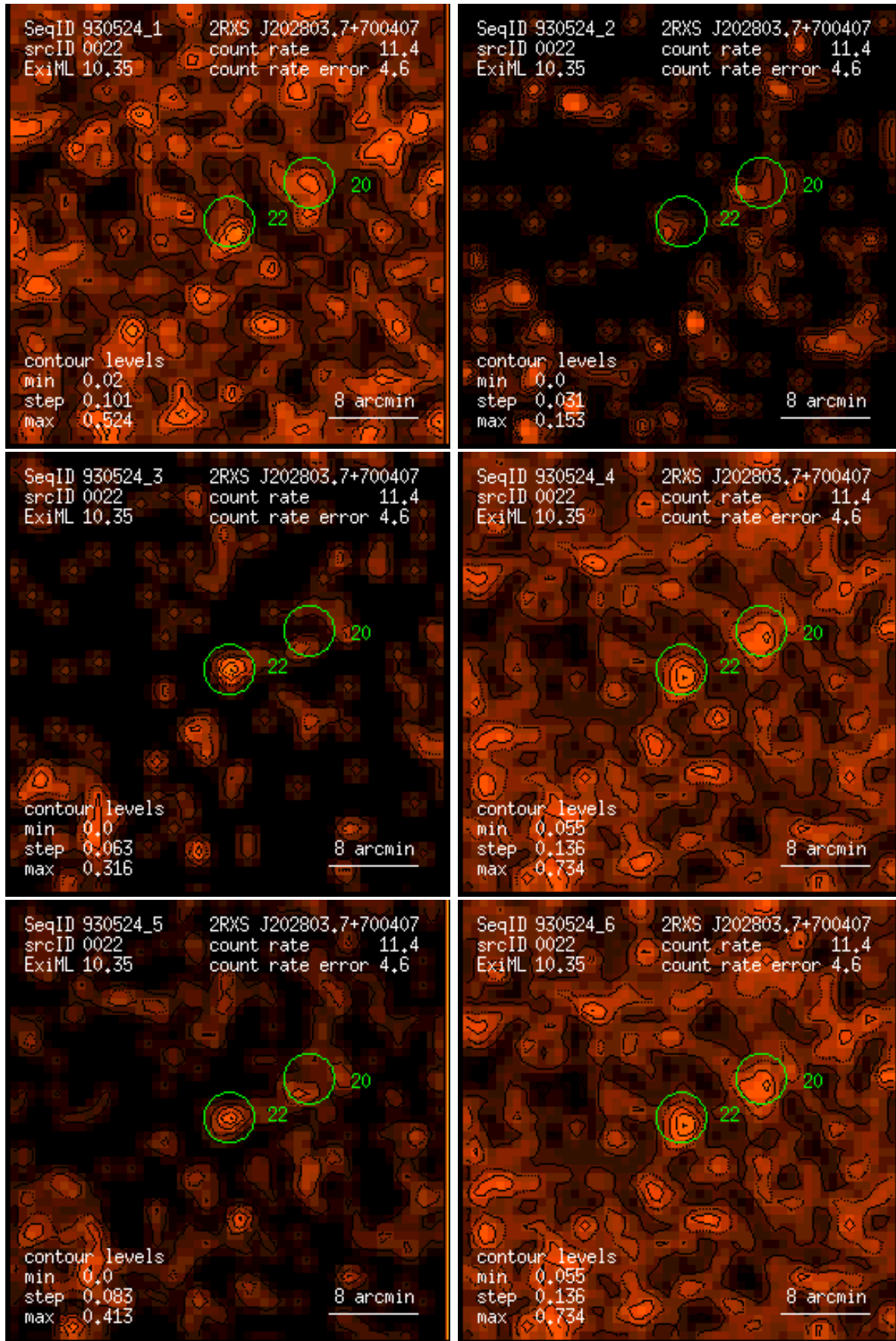
Figure 22: RASS 930524: detection 0022: band rate images, Gaussian filter: (1) PSPC channels 11 – 41, (2) 52 – 90, (3) 91 – 201, (4) 11 – 235, (5) 52 – 201, (6) 11 – 201. Broad band rates in counts/ks. Band rate contour levels in counts/ks/arcmin 2 .
