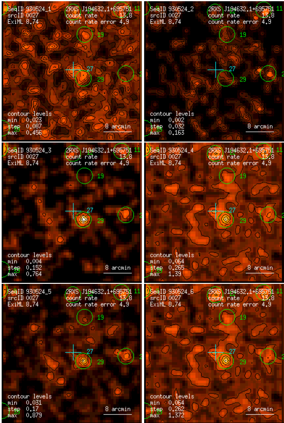
Figure 27: RASS 930524: detection 0027: band rate images, Gaussian filter: (1) PSPC channels 11 – 41, (2) 52 – 90, (3) 91 – 201, (4) 11 – 235, (5) 52 – 201, (6) 11 – 201. Broad band rates in counts/ks. Band rate contour levels in counts/ks/arcmin 2 .
