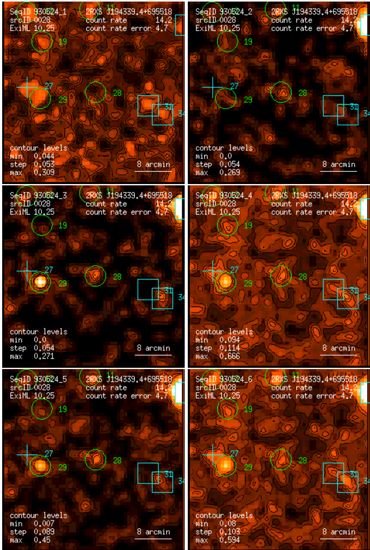
Figure 28: RASS 930524: detection 0028: band rate images, Gaussian filter: (1) PSPC channels 11 – 41, (2) 52 – 90, (3) 91 – 201, (4) 11 – 235, (5) 52 – 201, (6) 11 – 201. Broad band rates in counts/ks. Band rate contour levels in counts/ks/arcmin 2 .
