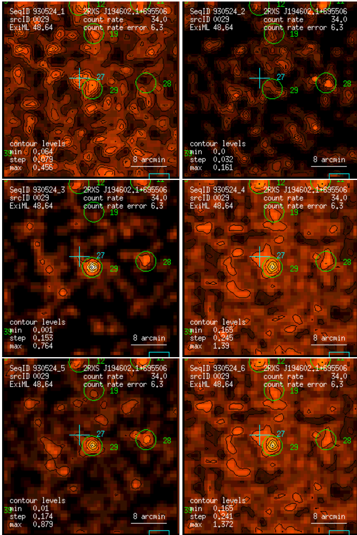
Figure 29: RASS 930524: detection 0029: band rate images, Gaussian filter: (1) PSPC channels 11 – 41, (2) 52 – 90, (3) 91 – 201, (4) 11 – 235, (5) 52 – 201, (6) 11 – 201. Broad band rates in counts/ks. Band rate contour levels in counts/ks/arcmin 2 .
