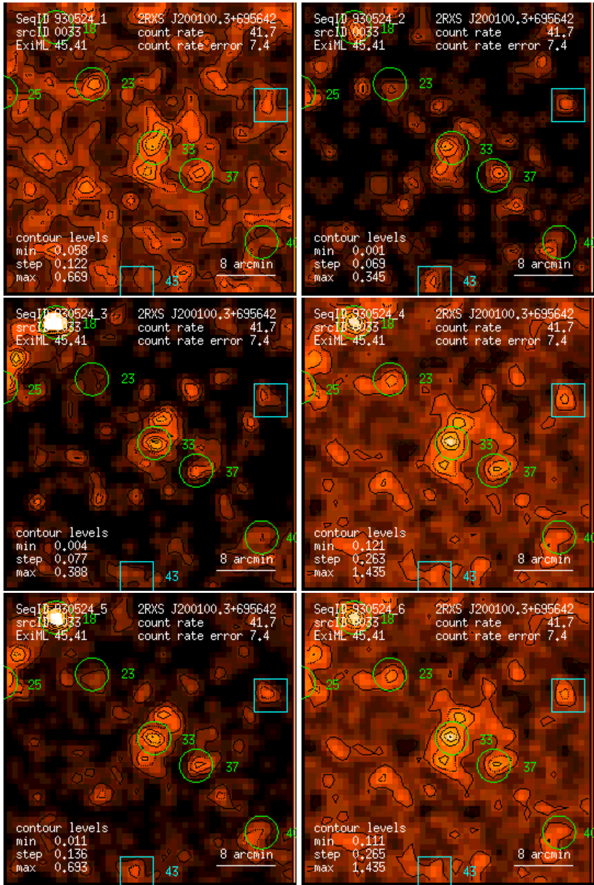
Figure 33: RASS 930524: detection 0033: band rate images, Gaussian filter: (1) PSPC channels 11 – 41, (2) 52 – 90, (3) 91 – 201, (4) 11 – 235, (5) 52 – 201, (6) 11 – 201. Broad band rates in counts/ks. Band rate contour levels in counts/ks/arcmin 2 .
