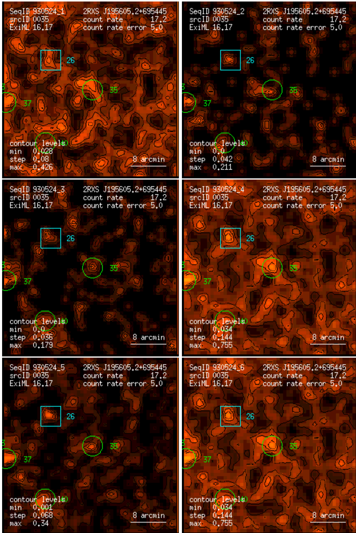
Figure 35: RASS 930524: detection 0035: band rate images, Gaussian filter: (1) PSPC channels 11 – 41, (2) 52 – 90, (3) 91 – 201, (4) 11 – 235, (5) 52 – 201, (6) 11 – 201. Broad band rates in counts/ks. Band rate contour levels in counts/ks/arcmin 2 .
