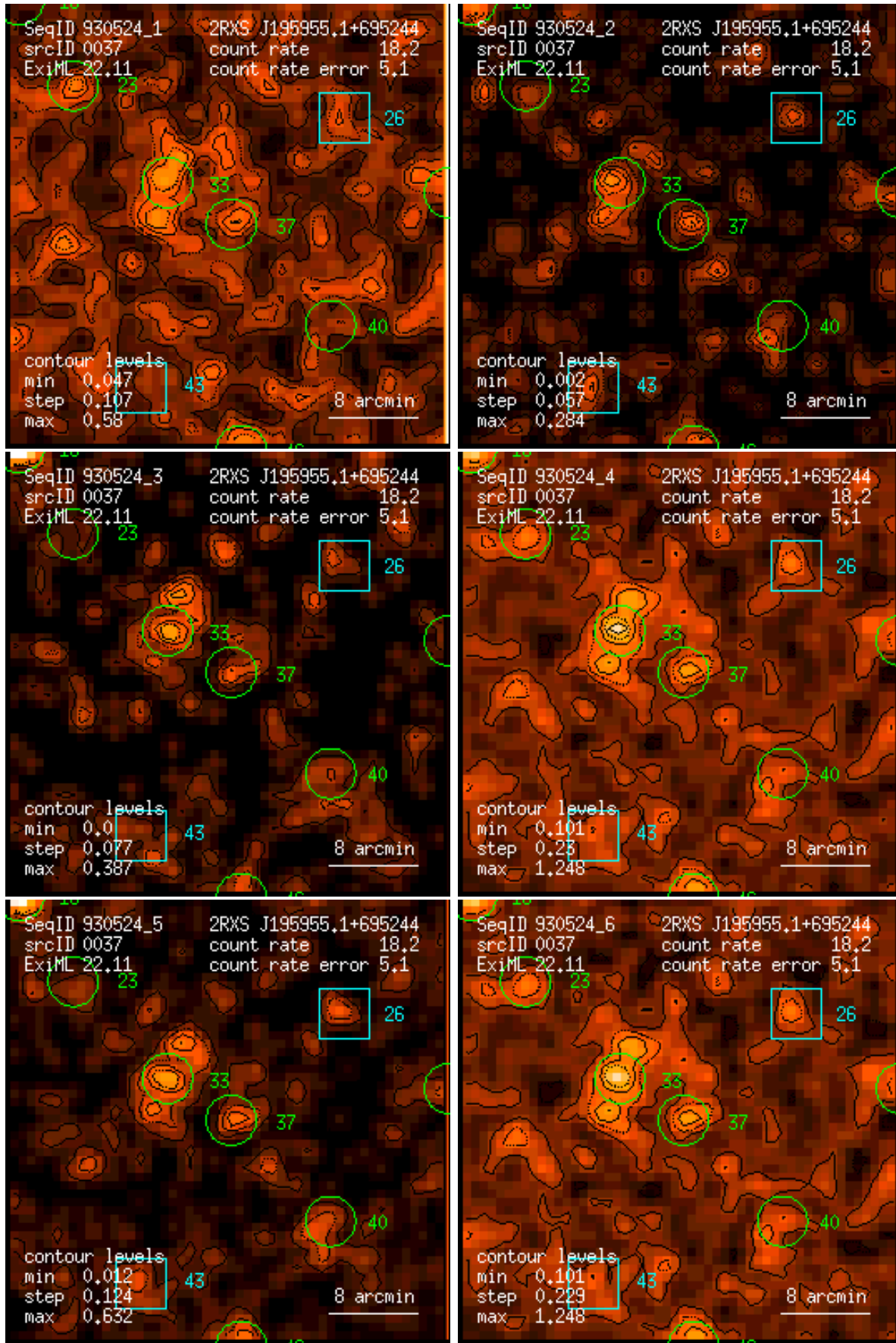
Figure 37: RASS 930524: detection 0037: band rate images, Gaussian filter: (1) PSPC channels 11 – 41, (2) 52 – 90, (3) 91 – 201, (4) 11 – 235, (5) 52 – 201, (6) 11 – 201. Broad band rates in counts/ks. Band rate contour levels in counts/ks/arcmin 2 .
