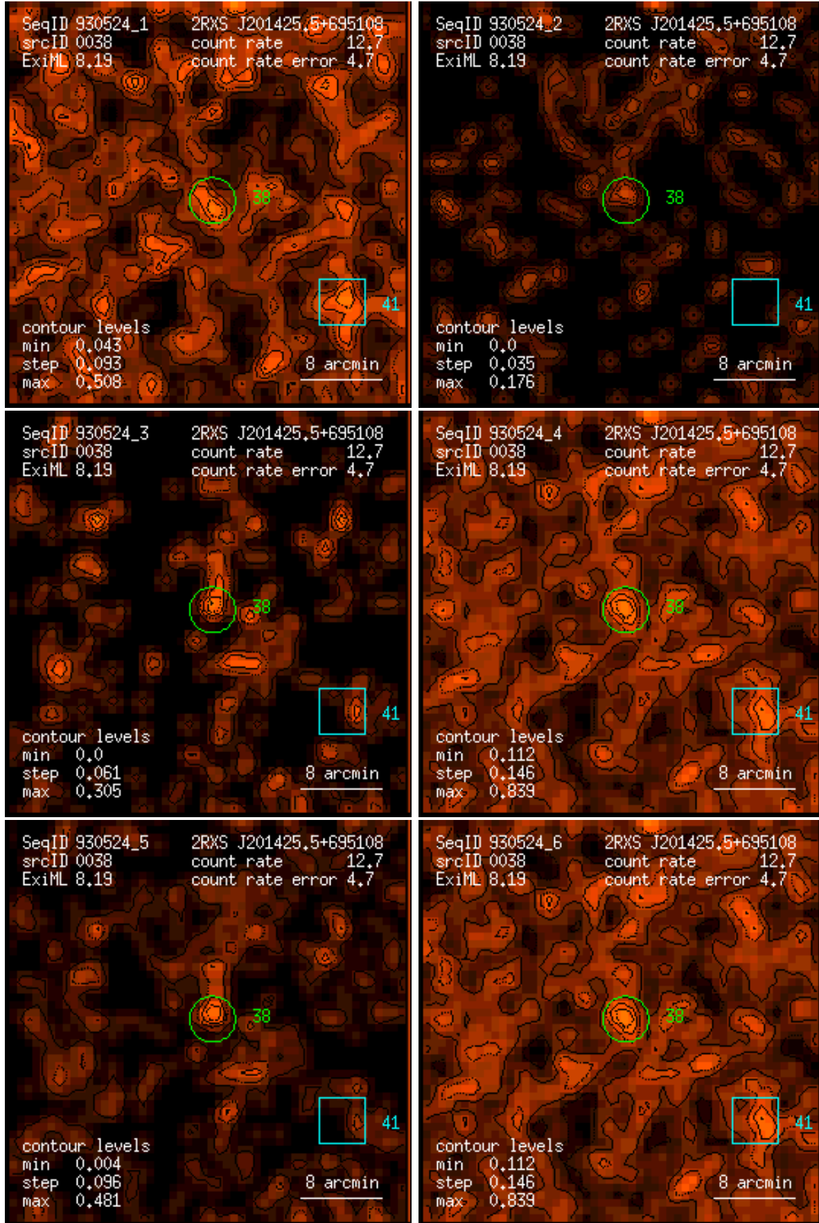
Figure 38: RASS 930524: detection 0038: band rate images, Gaussian filter: (1) PSPC channels 11 – 41, (2) 52 – 90, (3) 91 – 201, (4) 11 – 235, (5) 52 – 201, (6) 11 – 201. Broad band rates in counts/ks. Band rate contour levels in counts/ks/arcmin 2 .
