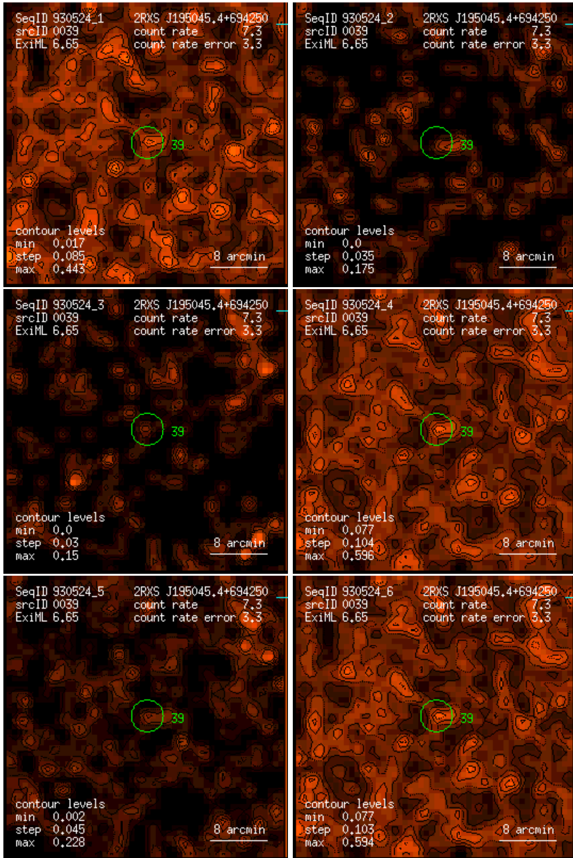
Figure 39: RASS 930524: detection 0039: band rate images, Gaussian filter: (1) PSPC channels 11 – 41, (2) 52 – 90, (3) 91 – 201, (4) 11 – 235, (5) 52 – 201, (6) 11 – 201. Broad band rates in counts/ks. Band rate contour levels in counts/ks/arcmin 2 .
