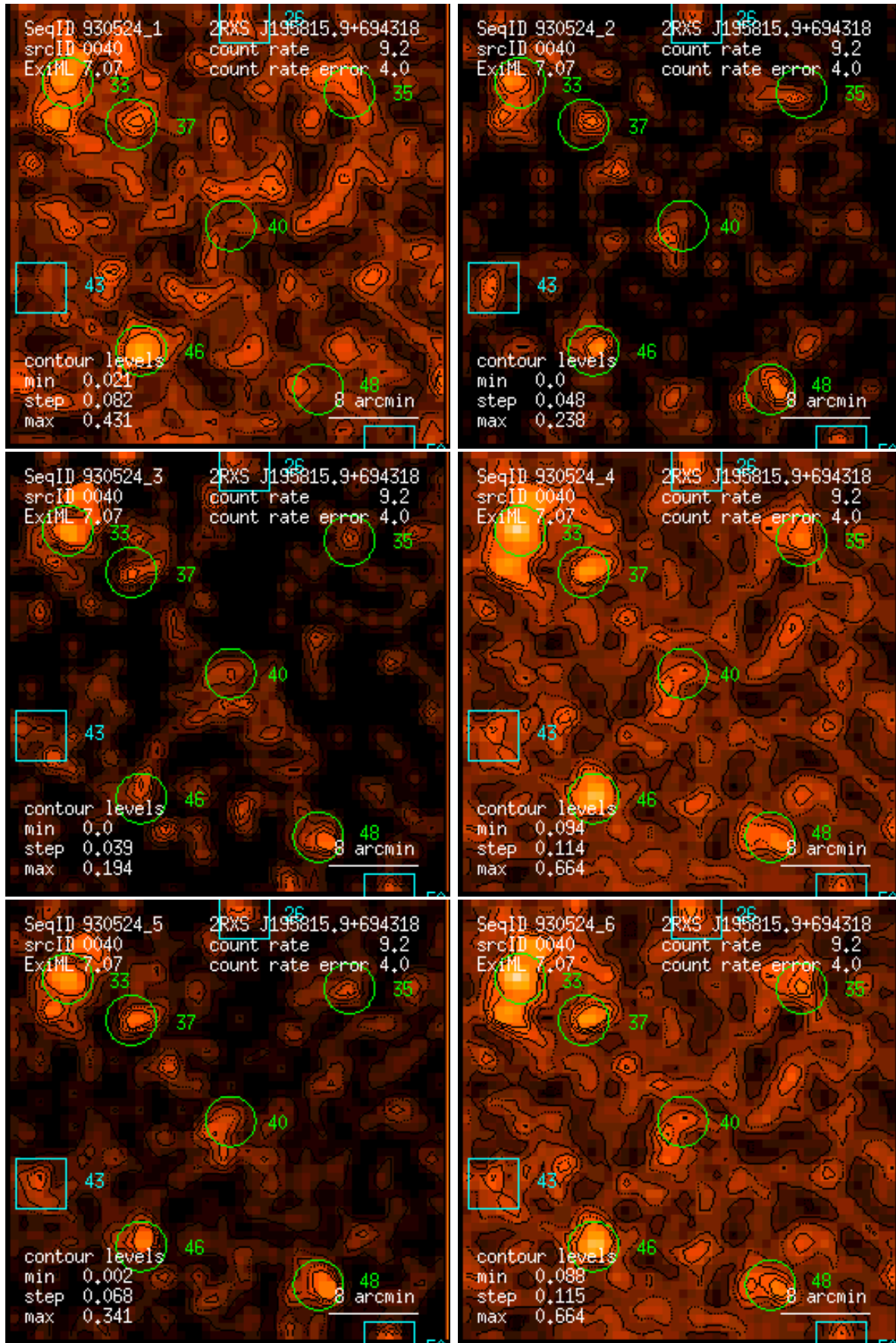
Figure 40: RASS 930524: detection 0040: band rate images, Gaussian filter: (1) PSPC channels 11 – 41, (2) 52 – 90, (3) 91 – 201, (4) 11 – 235, (5) 52 – 201, (6) 11 – 201. Broad band rates in counts/ks. Band rate contour levels in counts/ks/arcmin 2 .
