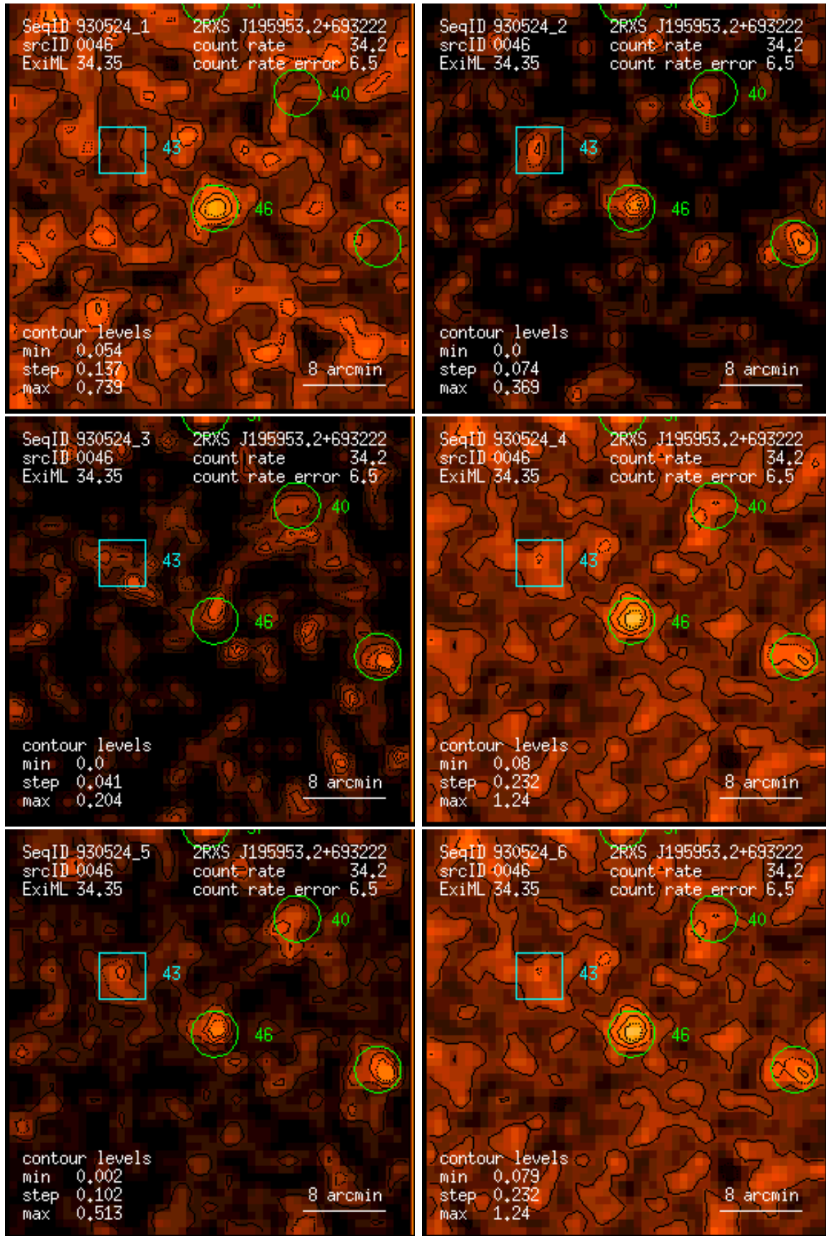
Figure 46: RASS 930524: detection 0046: band rate images, Gaussian filter: (1) PSPC channels 11 – 41, (2) 52 – 90, (3) 91 – 201, (4) 11 – 235, (5) 52 – 201, (6) 11 – 201. Broad band rates in counts/ks. Band rate contour levels in counts/ks/arcmin 2 .
