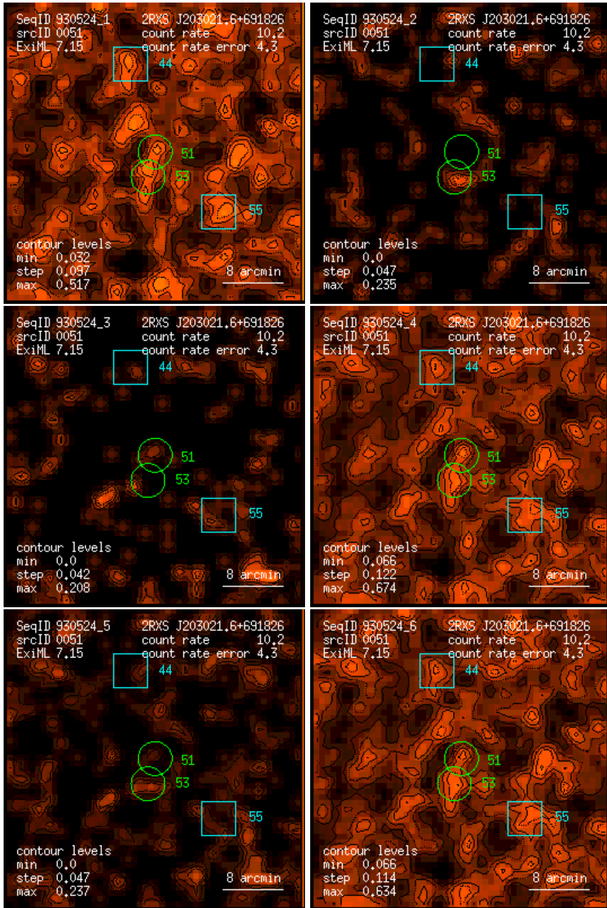
Figure 51: RASS 930524: detection 0051: band rate images, Gaussian filter: (1) PSPC channels 11 – 41, (2) 52 – 90, (3) 91 – 201, (4) 11 – 235, (5) 52 – 201, (6) 11 – 201. Broad band rates in counts/ks. Band rate contour levels in counts/ks/arcmin 2 .
