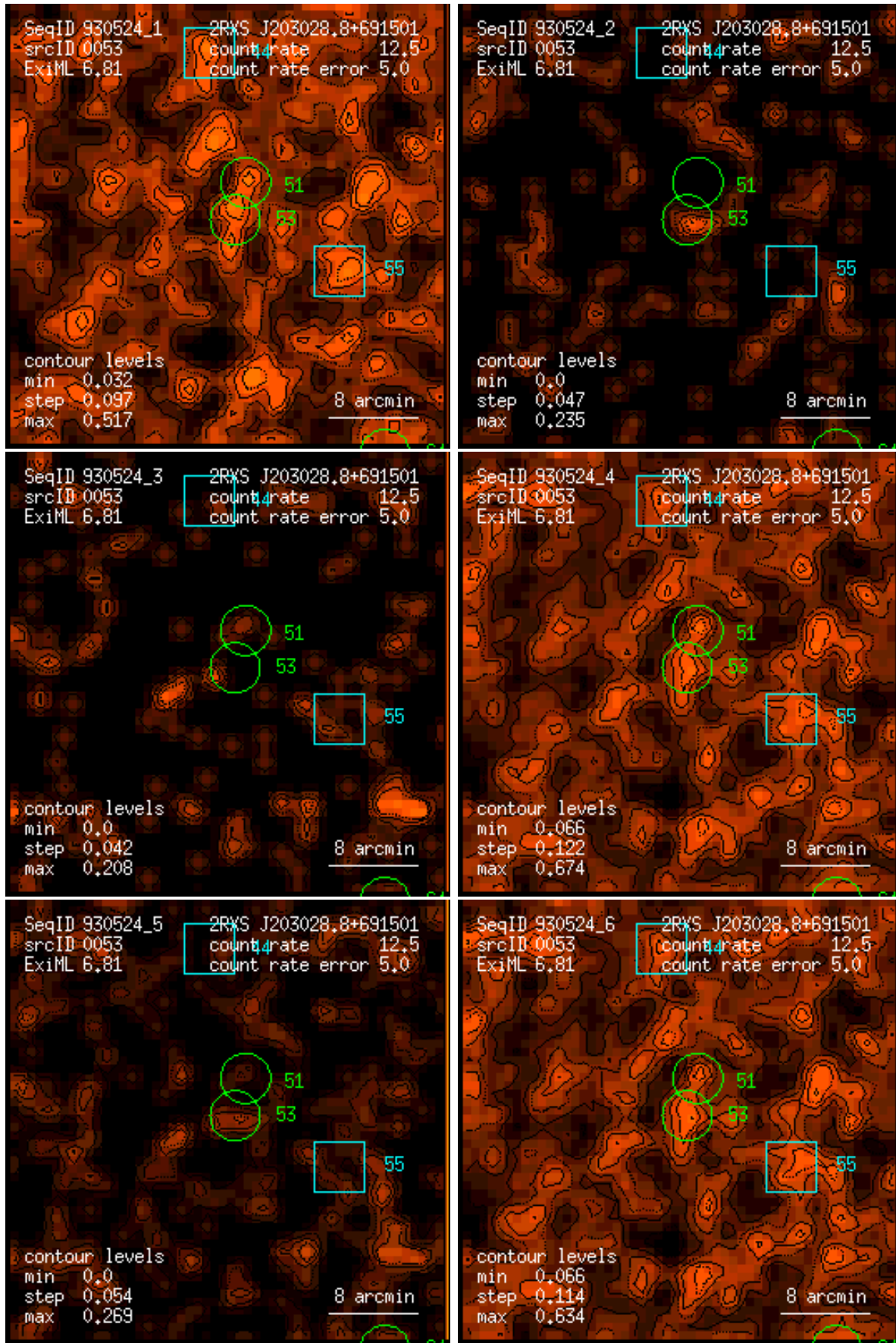
Figure 53: RASS 930524: detection 0053: band rate images, Gaussian filter: (1) PSPC channels 11 – 41, (2) 52 – 90, (3) 91 – 201, (4) 11 – 235, (5) 52 – 201, (6) 11 – 201. Broad band rates in counts/ks. Band rate contour levels in counts/ks/arcmin 2 .
